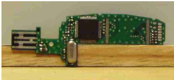
USB PCB component side (without Flash memory)
