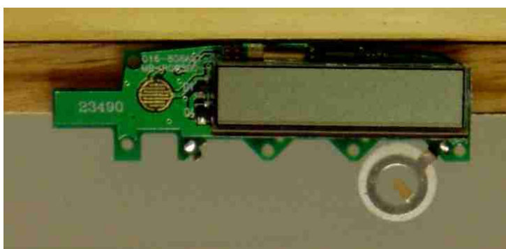
Display/Key/Batteries PCB
