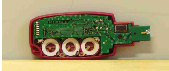
General view, cover opened (USB PCB copper side)
