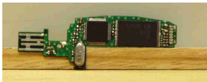
USB PCB component side (with Flash memory)
