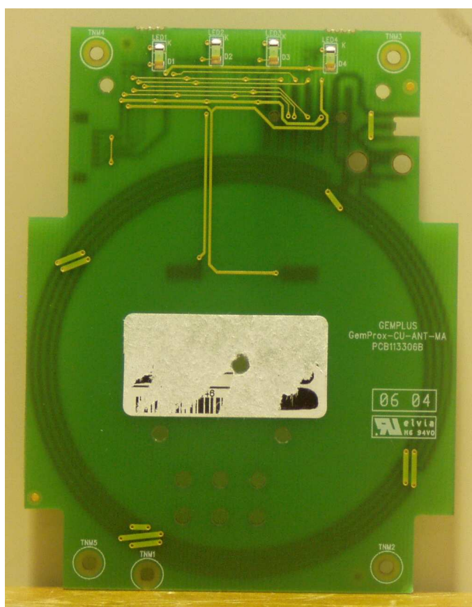
Antenna board
