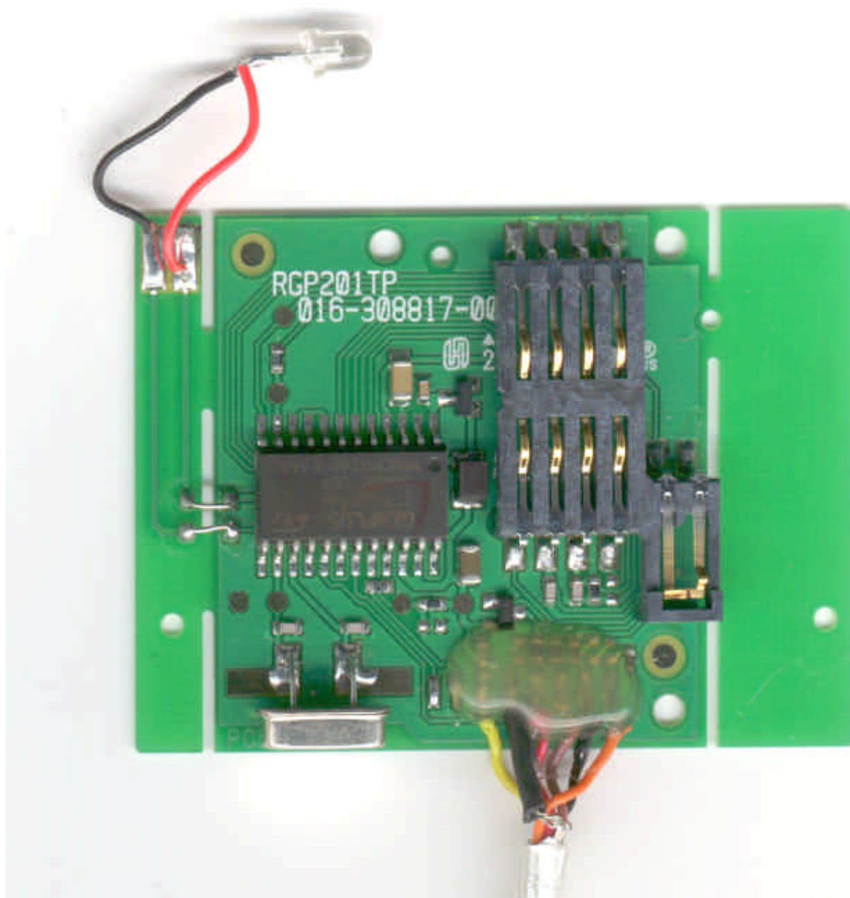
Internal board, Component side
