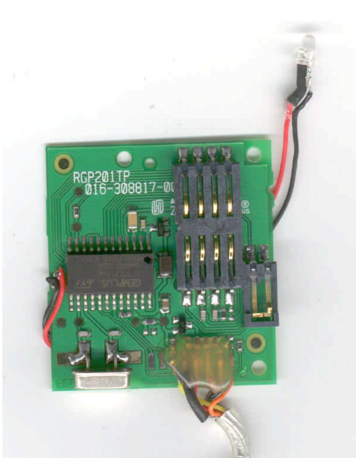
Internal board, Component side
