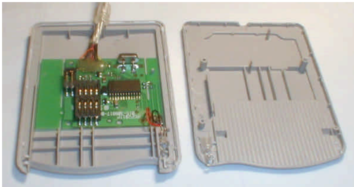
Internal view, Fences removed
