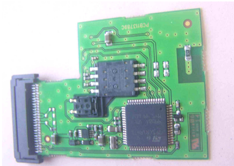
components side
