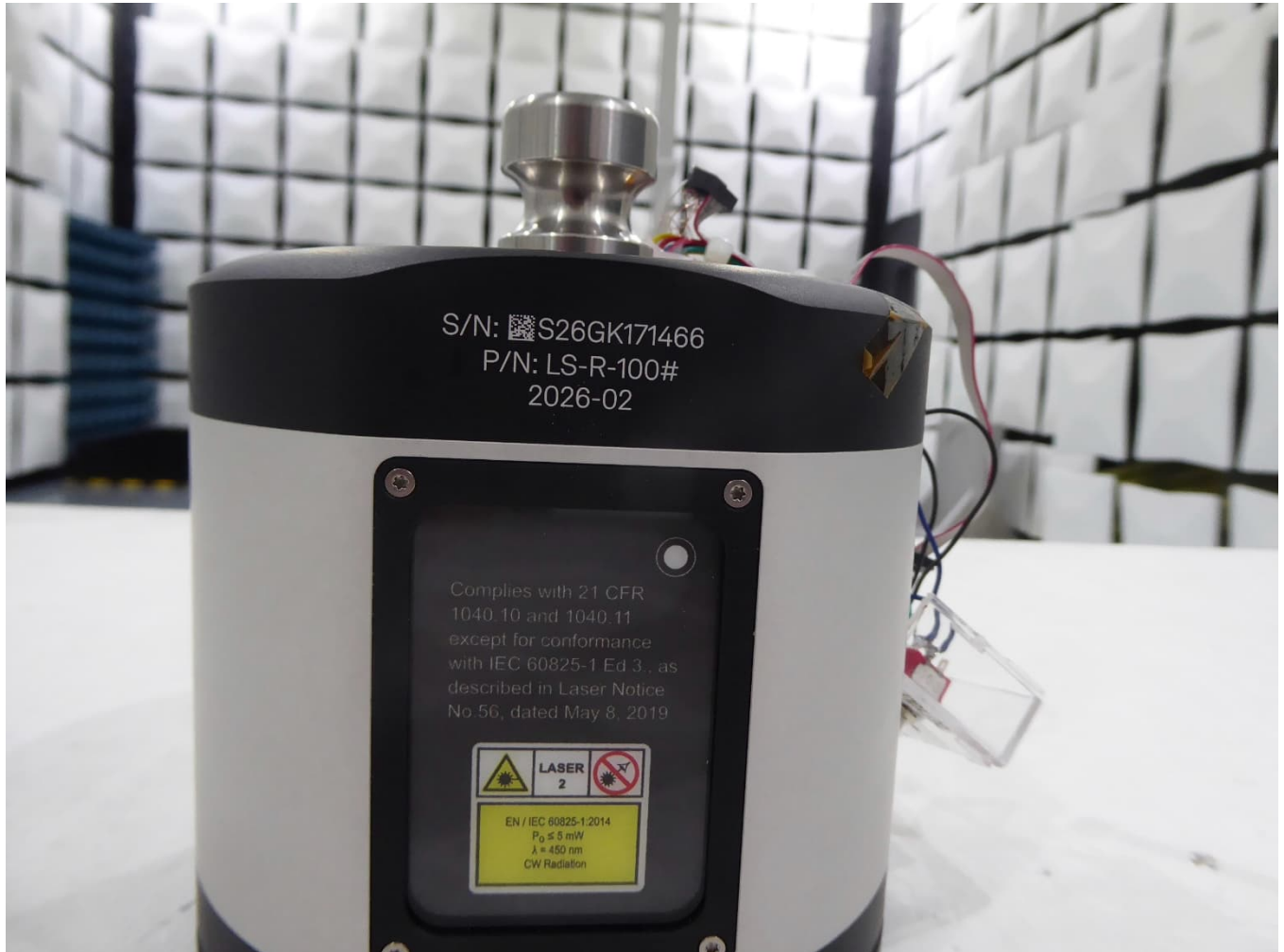
EUT Position 1 below 1GHz
