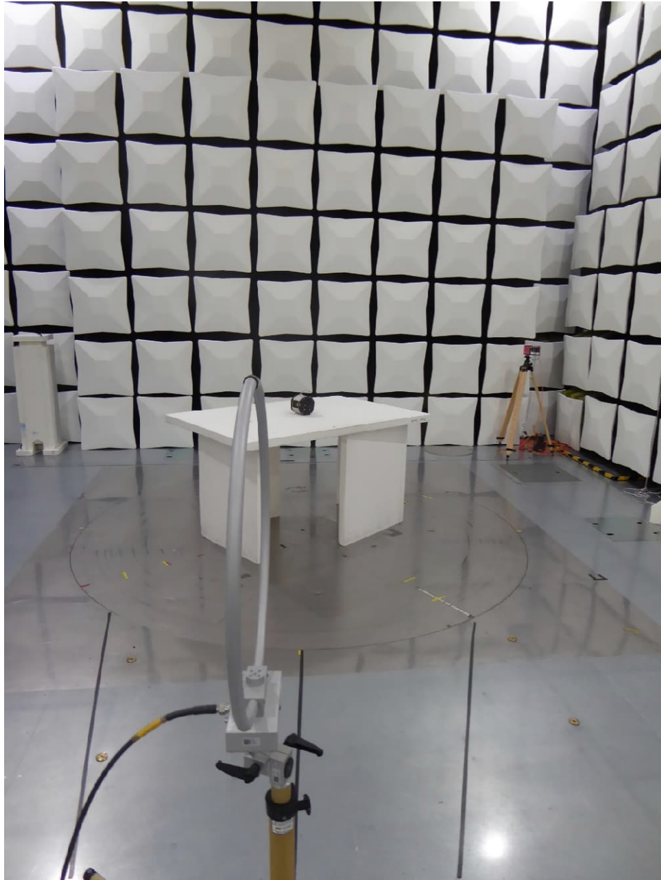
9 kHz – 30 MHz – Antenna Position 2
