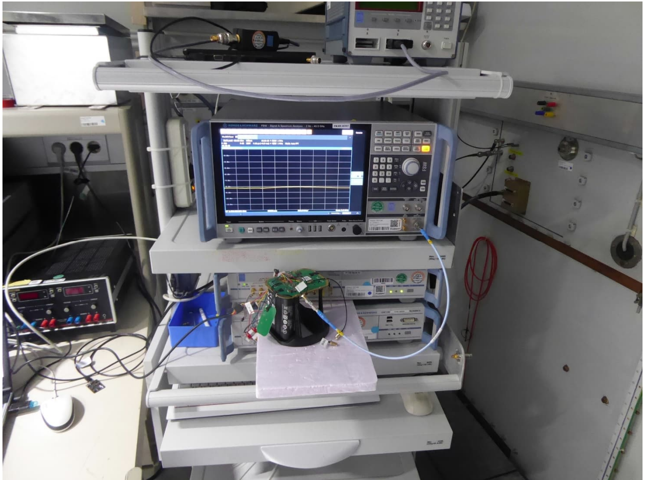
Conducted measurements
