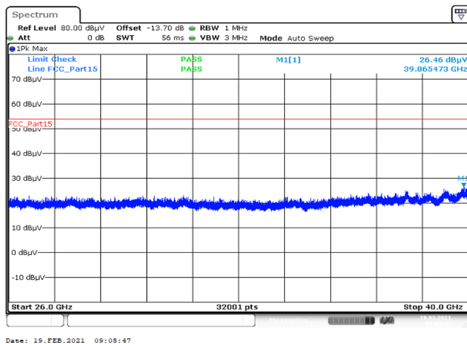
Plot 6: 26 GHz to 40 GHz; vertical & horizontal polarization; U-NII-1; mid channel
