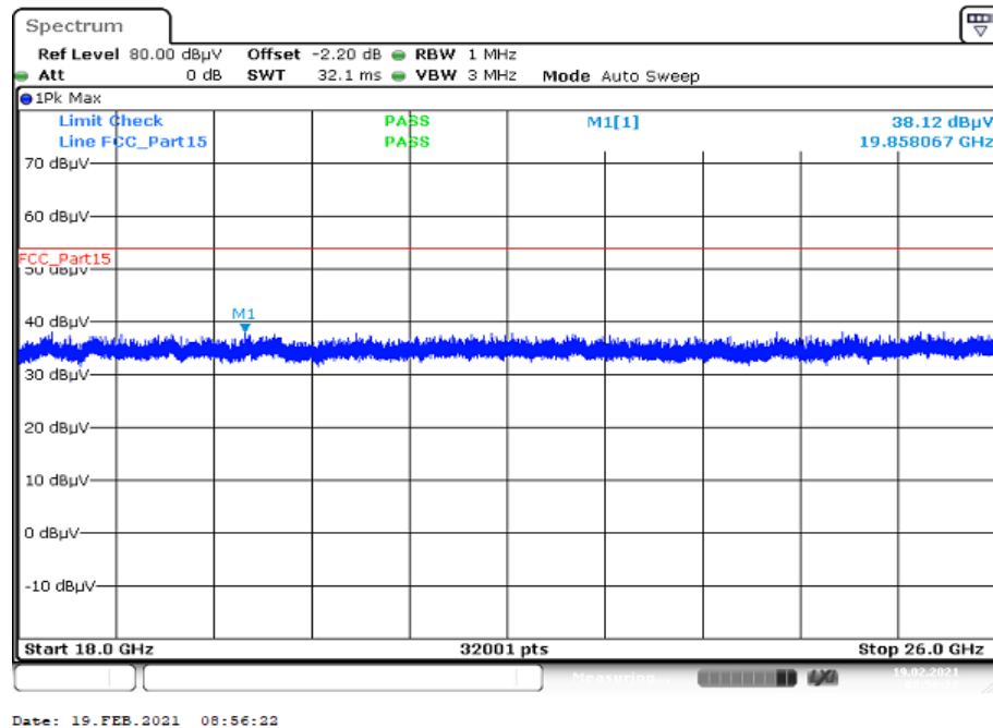
Plot 5: 18 GHz to 26 GHz; vertical & horizontal polarization; U-NII-1; mid channel
