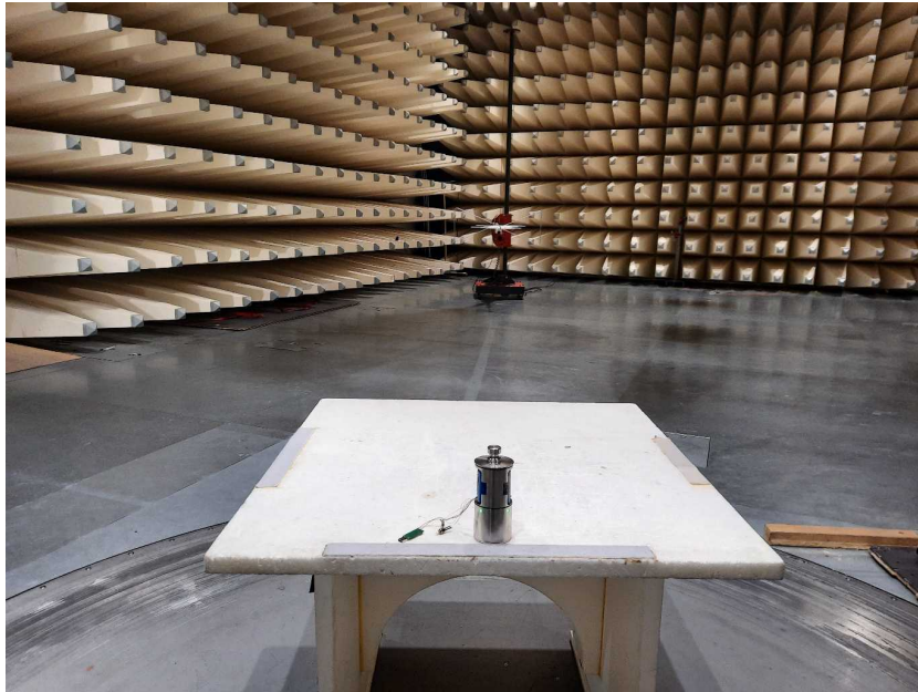
Photo 7 RSE < 1GHz
