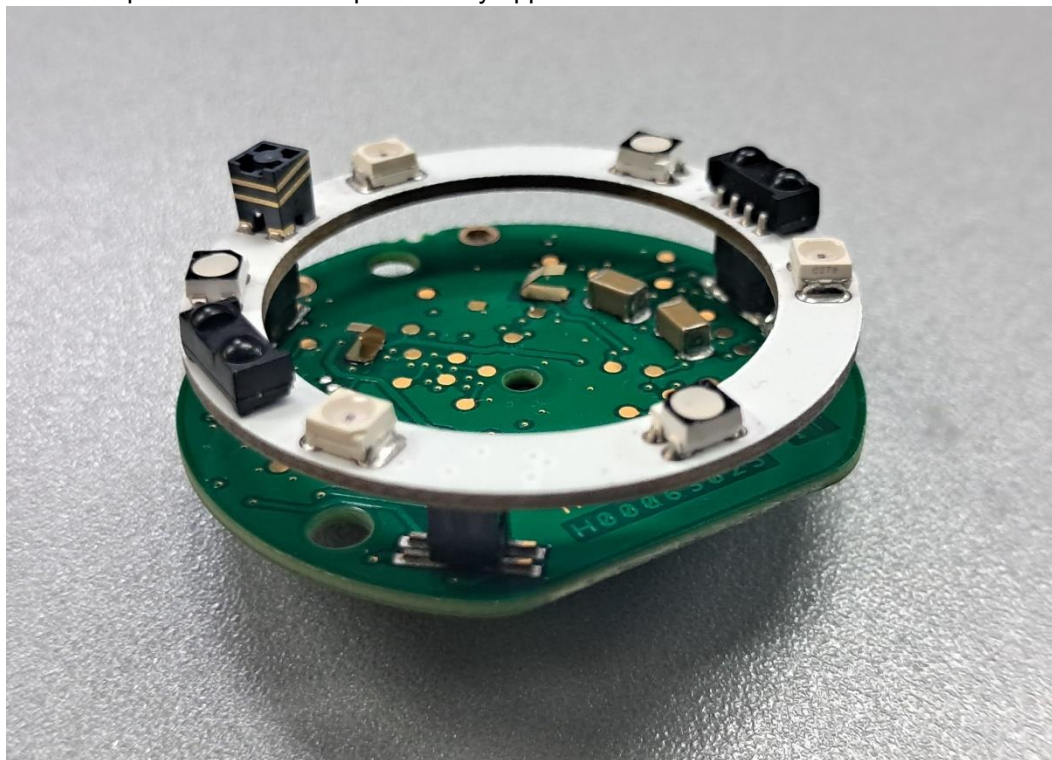
Photo No. 14: internal pictures of EUT as provided by applicant
