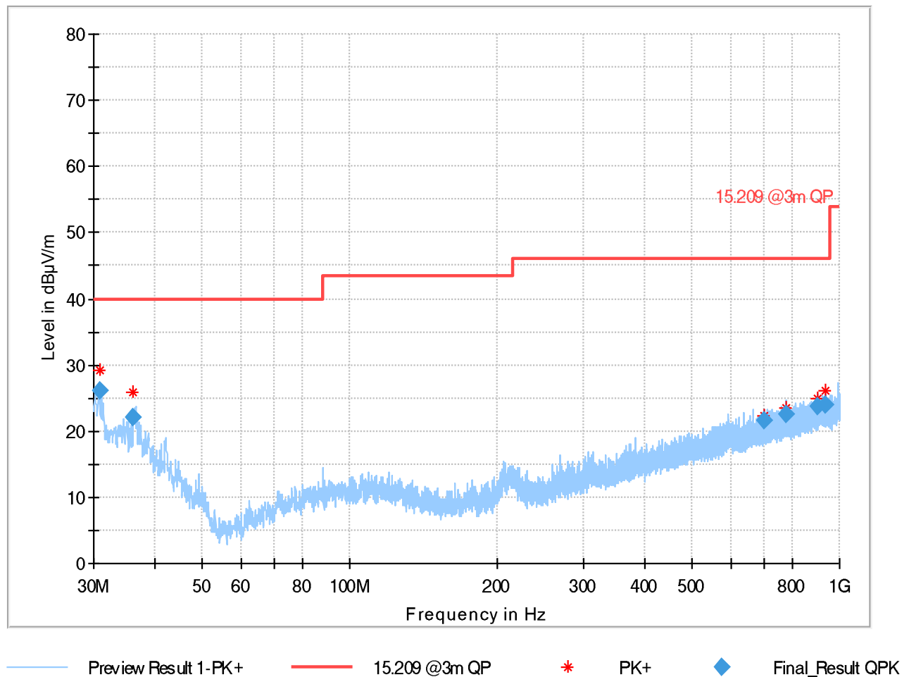
Plot 25: Mode 1, RSE 30 MHz – 1 GHz, high channel, horizontal / vertical polarisation
