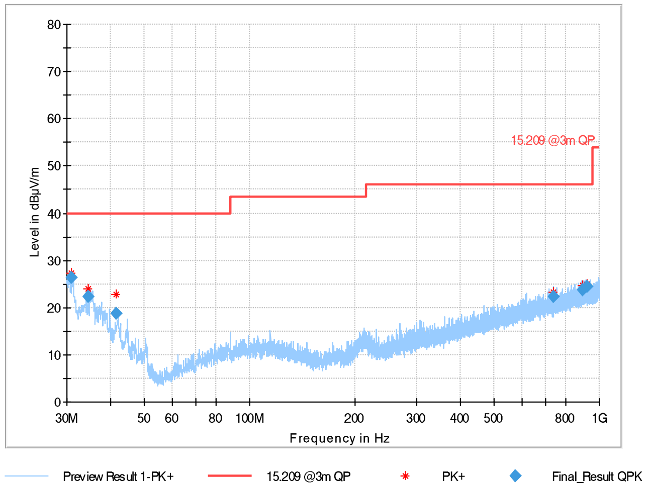
Plot 24: Mode 1, RSE 30 MHz – 1 GHz, mid channel, horizontal / vertical polarisation
