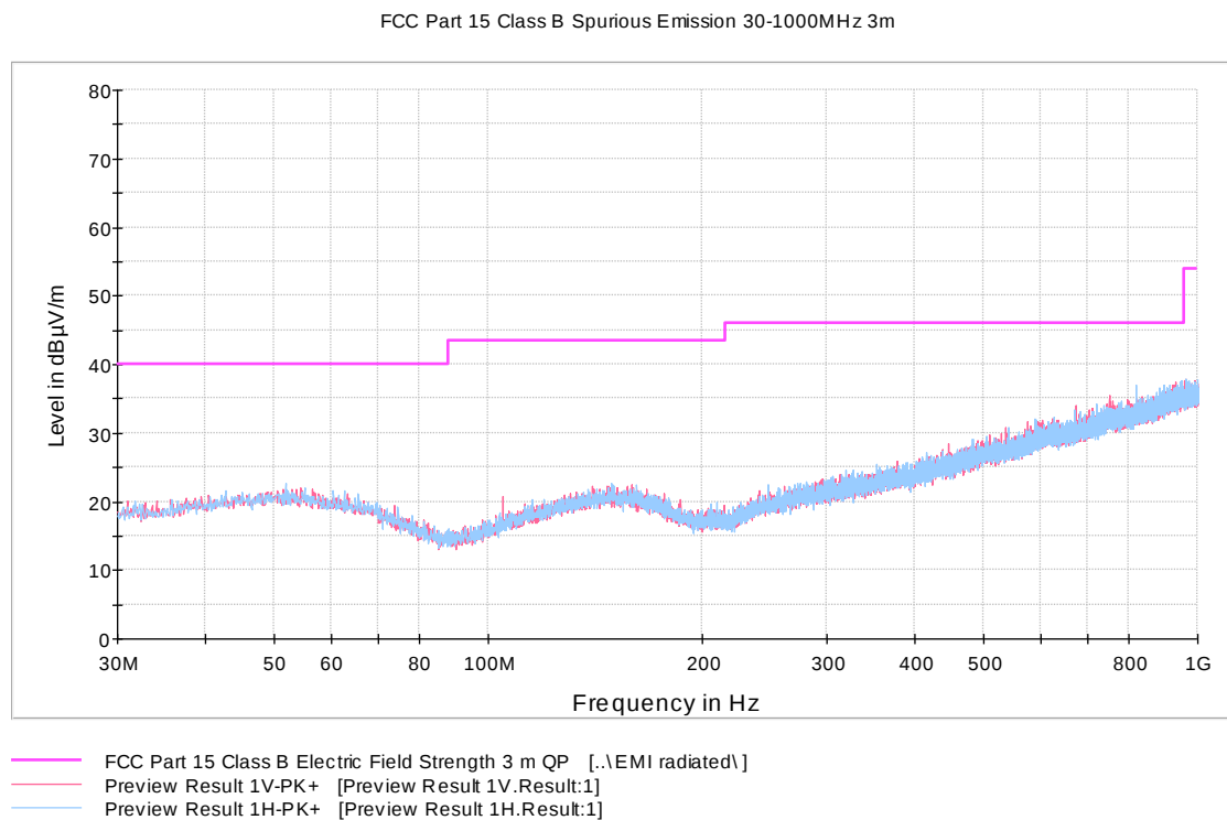
Figure 16: Channel 19 mid 30 MHz – 1000 MHz (A)
