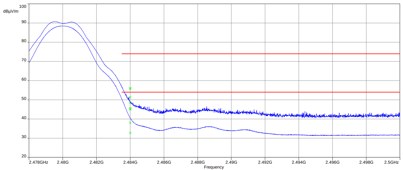
Plot 2: Upper restricted band
