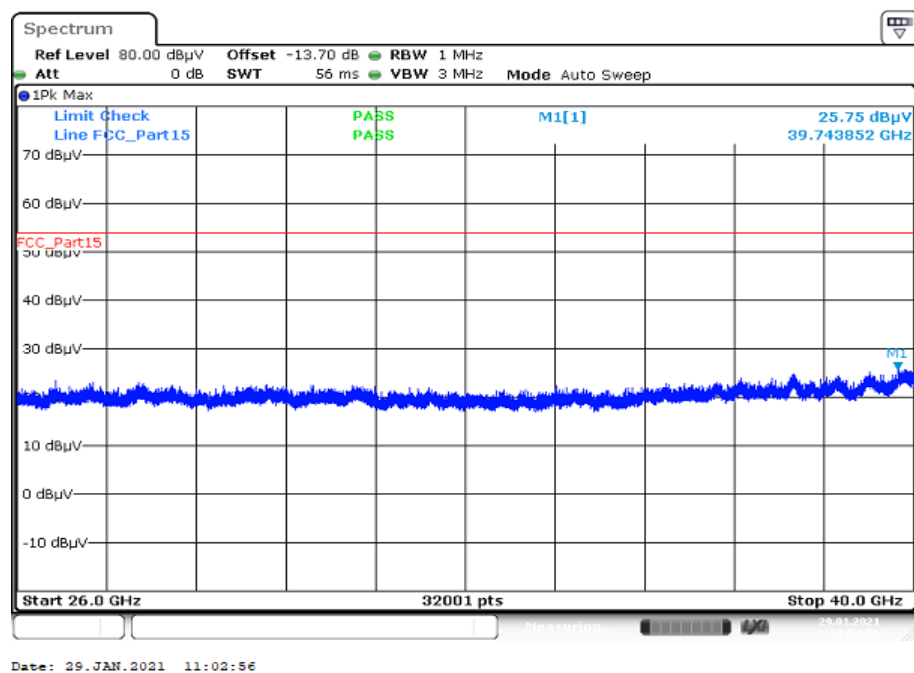
Plot 3: 26 GHz to 40 GHz; vertical & horizontal polarization
