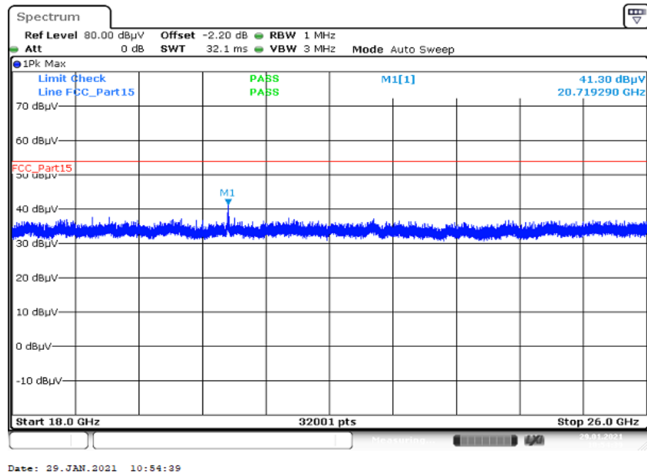
Plot 2: 18 GHz to 26 GHz; vertical & horizontal polarization
