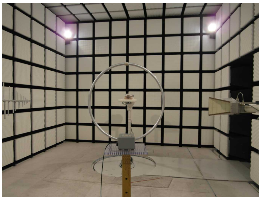
EUT at the anechoic chamber
