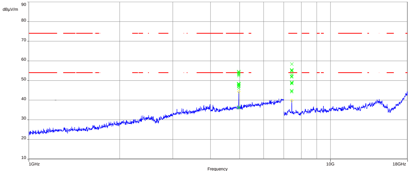
Plot 5: 1 GHz to 18 GHz, TX mode, 2480 MHz, vertical & horizontal polarization, Antenna 1
