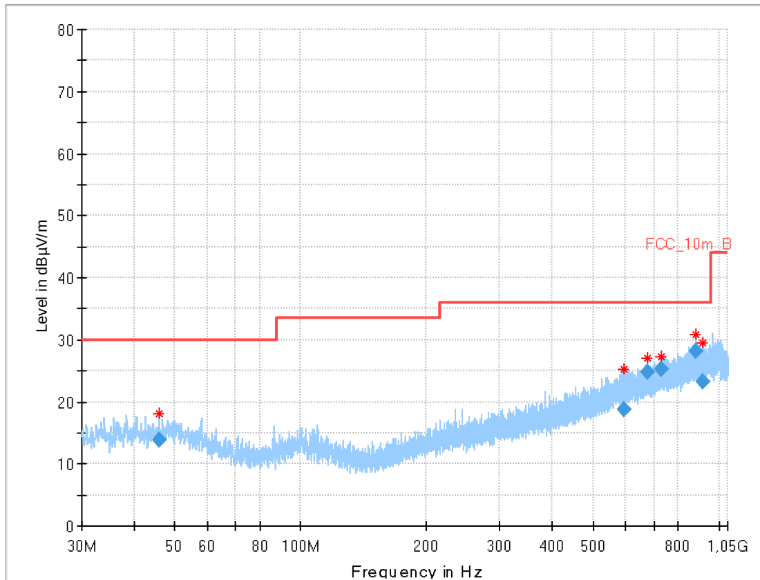
Plot 6: 30 MHz to 1 GHz, TX mode, 2480 MHz, vertical & horizontal polarization, Antenna 2
