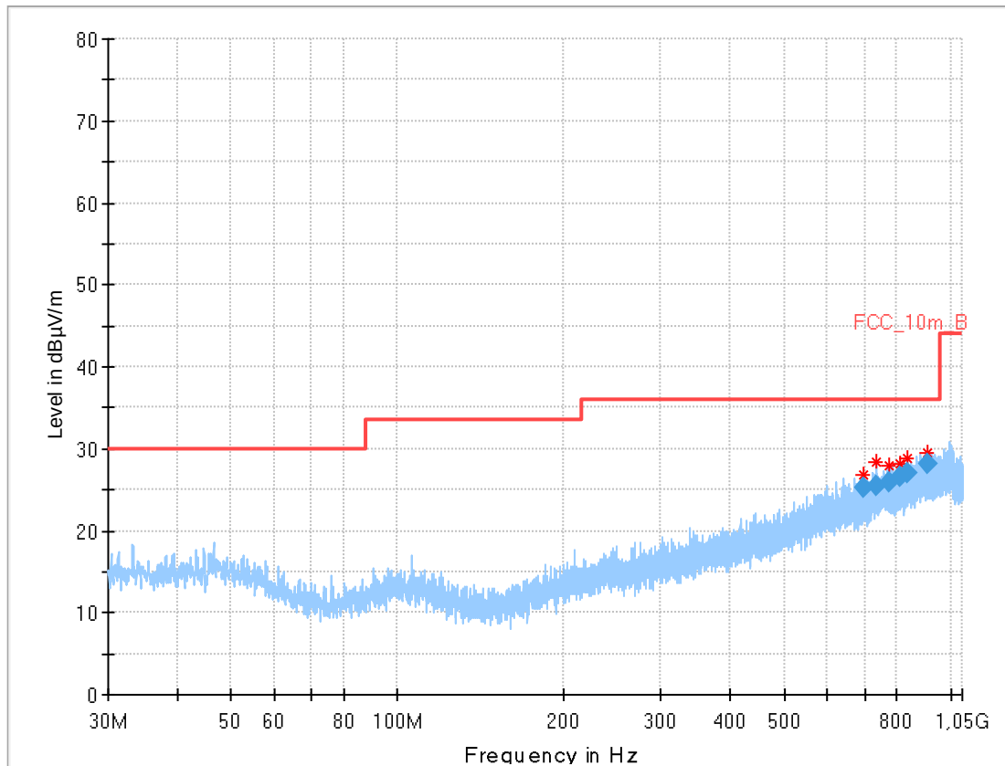
Plot 4: 30 MHz to 1 GHz, TX mode, 2405 MHz, vertical & horizontal polarization, Antenna 2
