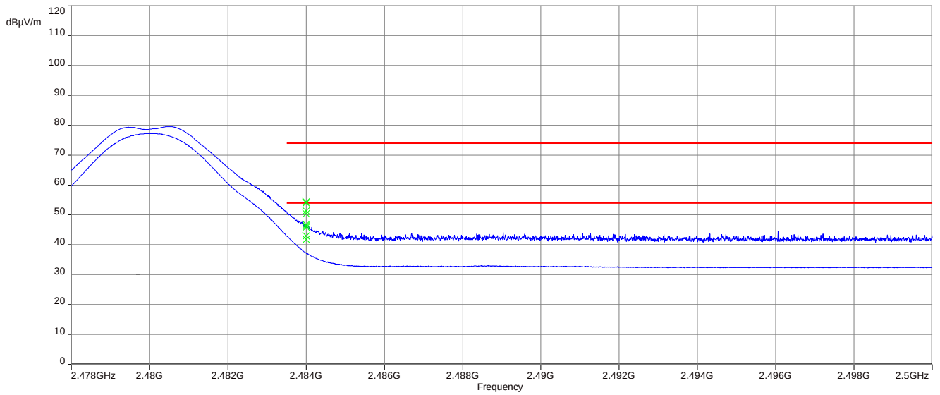
Plot 2: Upper restricted band, Antenna 1
