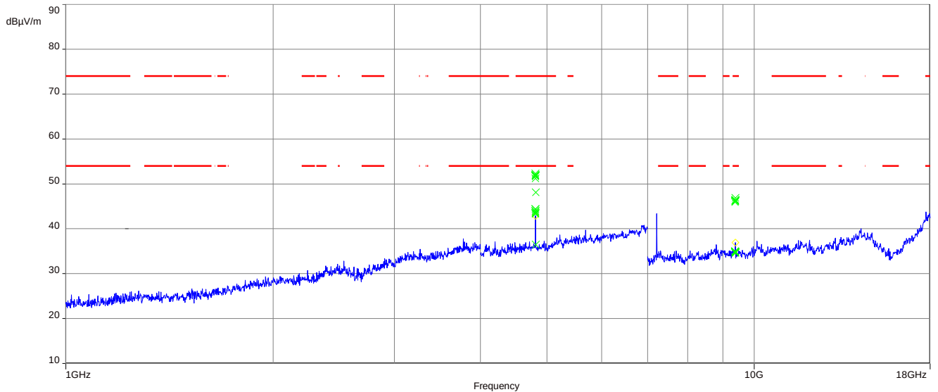
Plot 7: 1 GHz to 18 GHz, TX mode, 2405 MHz, vertical & horizontal polarization, Antenna 2
