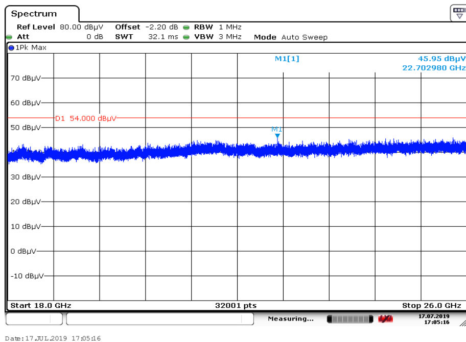
Plot 4: 18 GHz to 26 GHz, TX mode, 2440 MHz, vertical & horizontal polarization, Antenna 1
