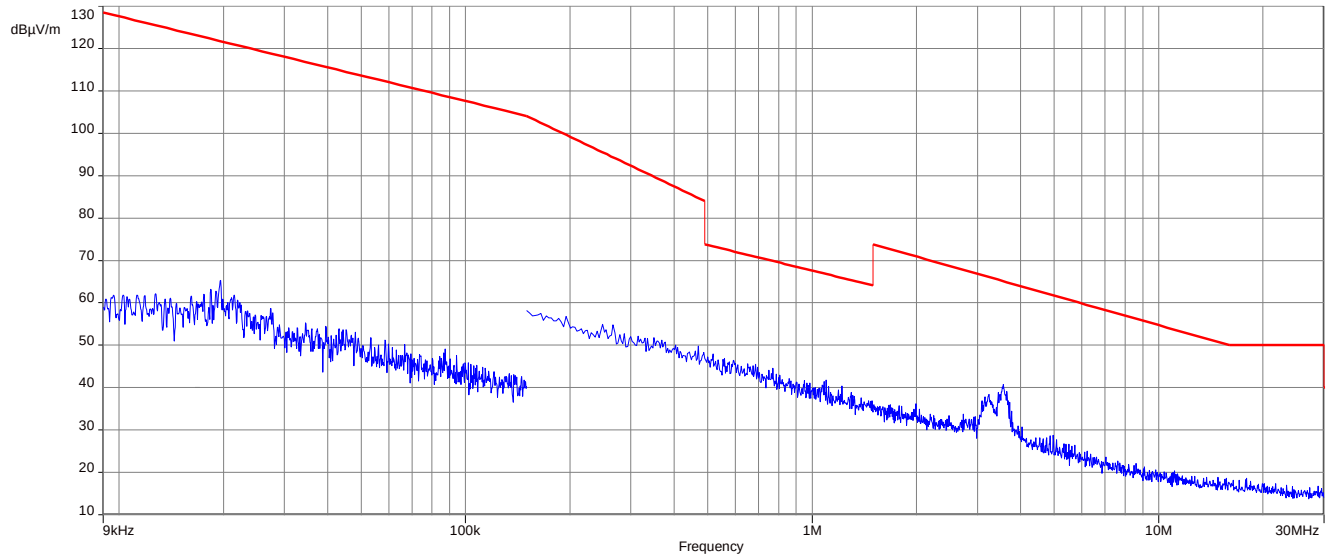
Plot 1: 9 kHz to 30 MHz, 2405 MHz, transmit mode, Antenna 1
