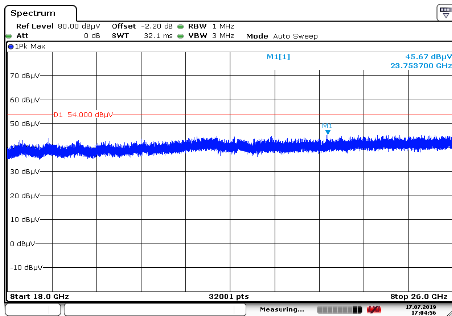
Plot 2: 18 GHz to 26 GHz, TX mode, 2405 MHz, vertical & horizontal polarization, Antenna 1
