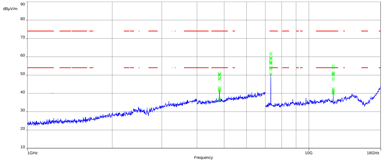
Plot 9: 1 GHz to 18 GHz, TX mode, 2440 MHz, vertical & horizontal polarization, Antenna 2
