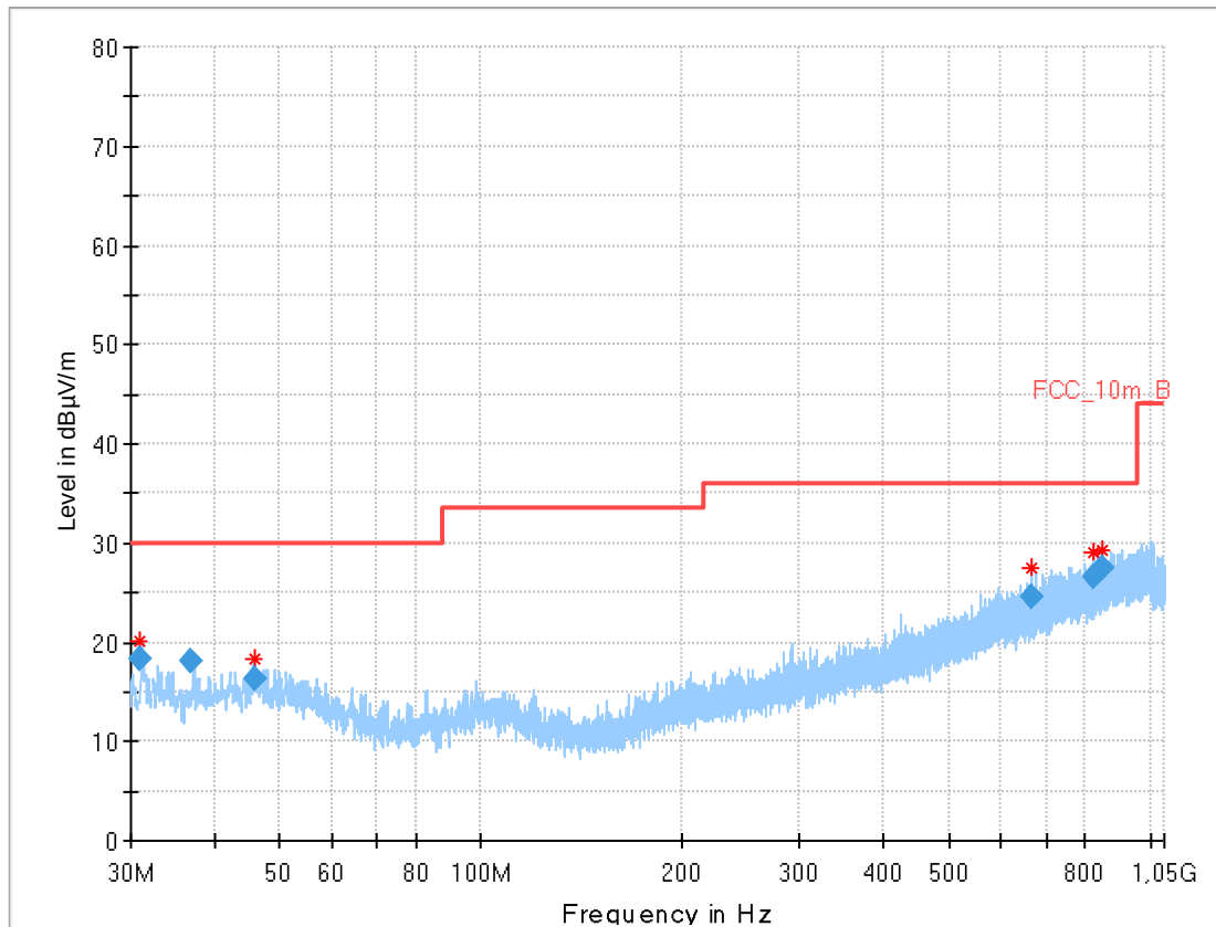
Plot 5: 30 MHz to 1 GHz, TX mode, 2440 MHz, vertical & horizontal polarization, Antenna 2
