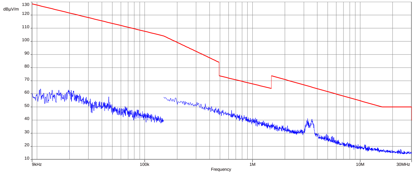
Plot 5: 9 kHz to 30 MHz, 2440 MHz, transmit mode, Antenna 2
