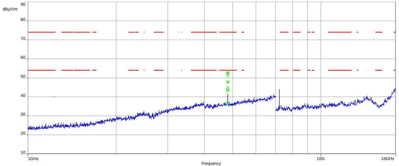
Plot 1: 1 GHz to 18 GHz, TX mode, 2405 MHz, vertical & horizontal polarization, Antenna 1
