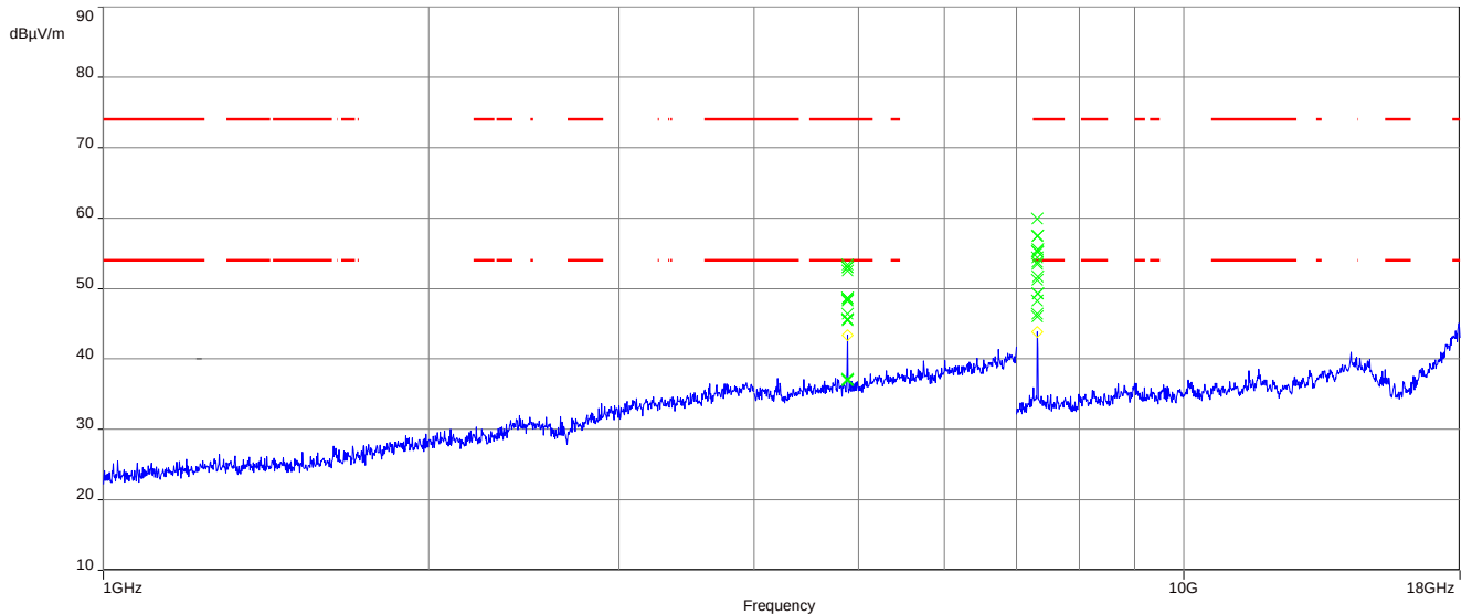
Plot 3: 1 GHz to 18 GHz, TX mode, 2440 MHz, vertical & horizontal polarization, Antenna 1
