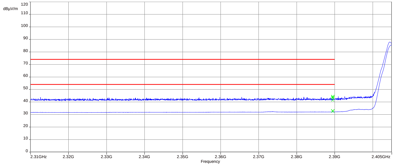
Plot 3: Lower restricted band, Antenna 2
