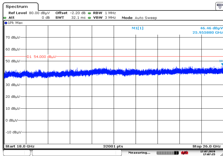
Plot 10: 18 GHz to 26 GHz, TX mode, 2440 MHz, vertical & horizontal polarization, Antenna 2
