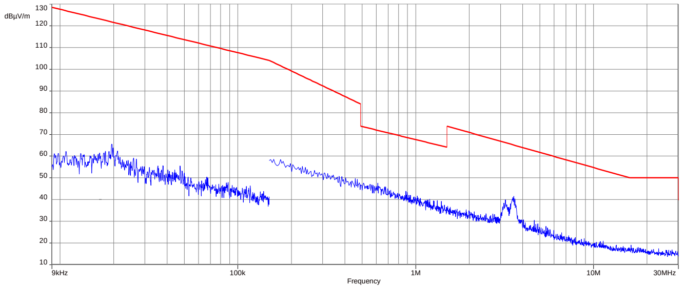
Plot 4: 9 kHz to 30 MHz, 2405 MHz, transmit mode, Antenna 2
