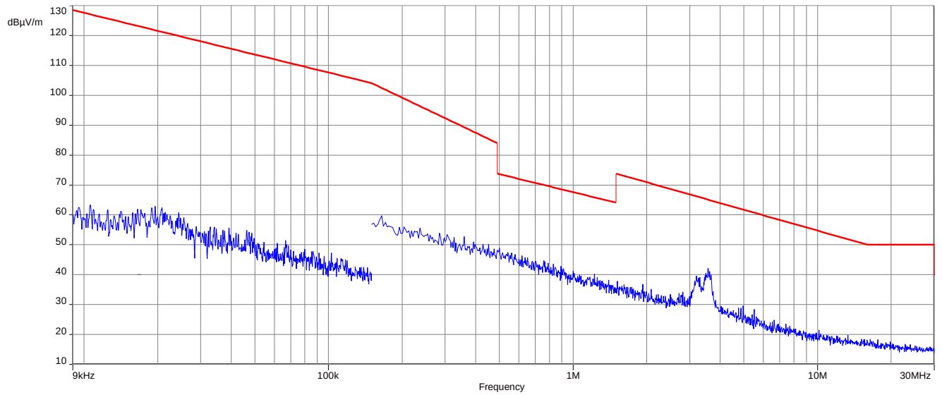
Plot 6: 9 kHz to 30 MHz, 2480 MHz, transmit mode, Antenna 2
