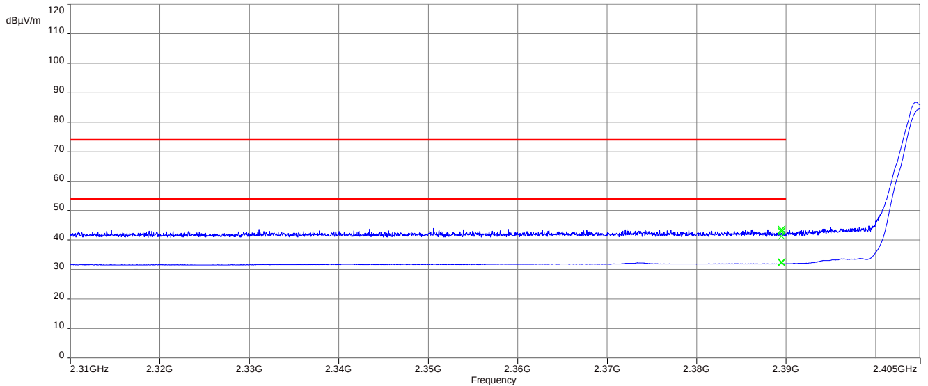
Plot 1: Lower restricted band, Antenna 1
