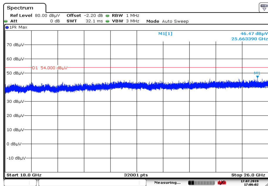
Plot 6: 18 GHz to 26 GHz, TX mode, 2480 MHz, vertical & horizontal polarization, Antenna 1
