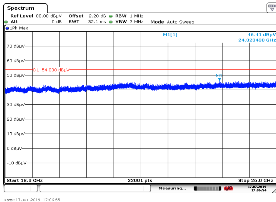
Plot 8: 18 GHz to 26 GHz, TX mode, 2405 MHz, vertical & horizontal polarization, Antenna 2
