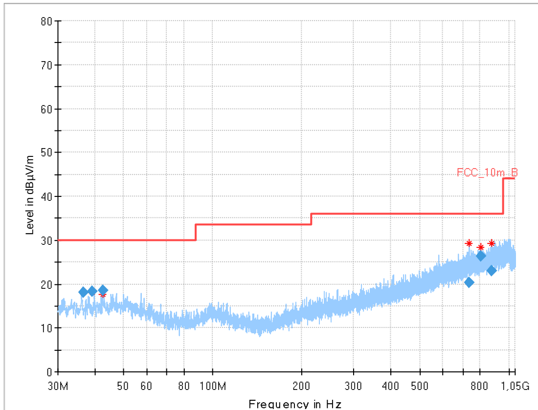
Plot 2: 30 MHz to 1 GHz, TX mode, 2440 MHz, vertical & horizontal polarization, Antenna 1
