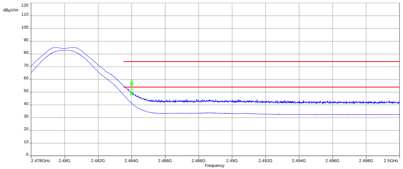
Plot 4: Upper restricted band, Antenna 2
