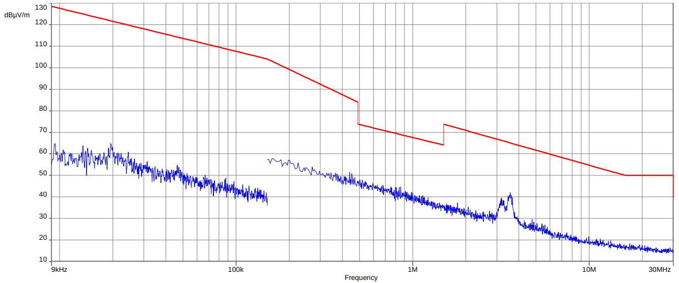
Plot 3: 9 kHz to 30 MHz, 2480 MHz, transmit mode, Antenna 1
