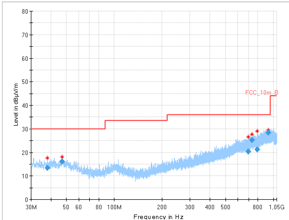
Plot 3: 30 MHz to 1 GHz, TX mode, 2480 MHz, vertical & horizontal polarization, Antenna 1
