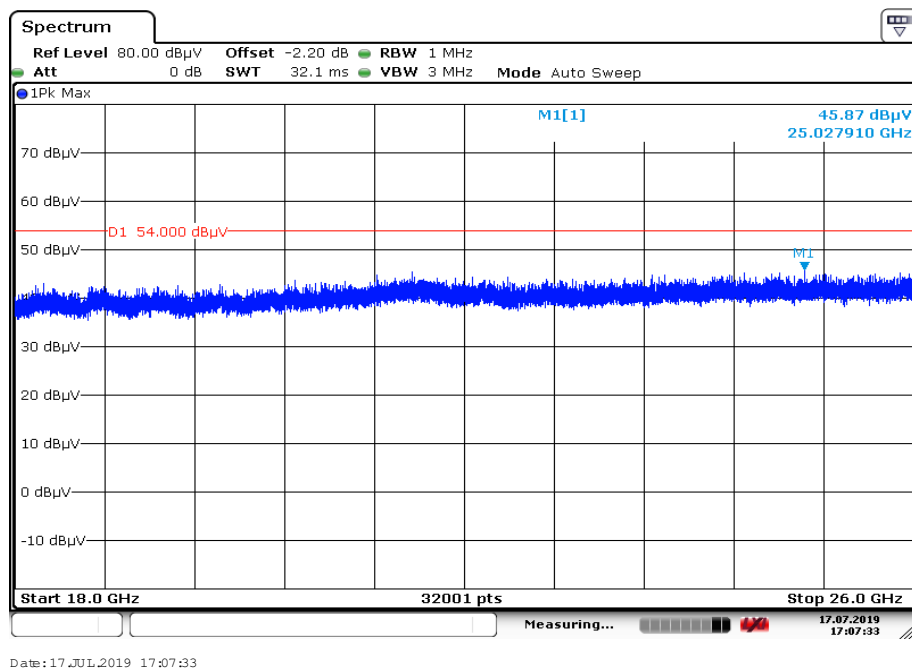
Plot 12: 18 GHz to 26 GHz, TX mode, 2480 MHz, vertical & horizontal polarization, Antenna 2
