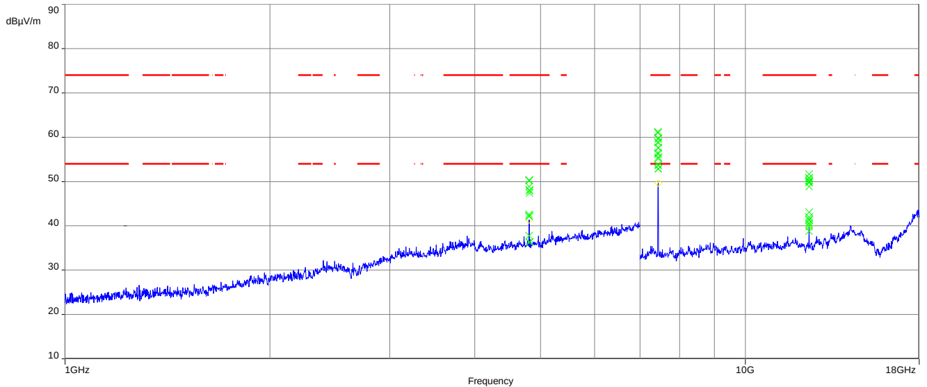
Plot 11: 1 GHz to 18 GHz, TX mode, 2480 MHz, vertical & horizontal polarization, Antenna 2
