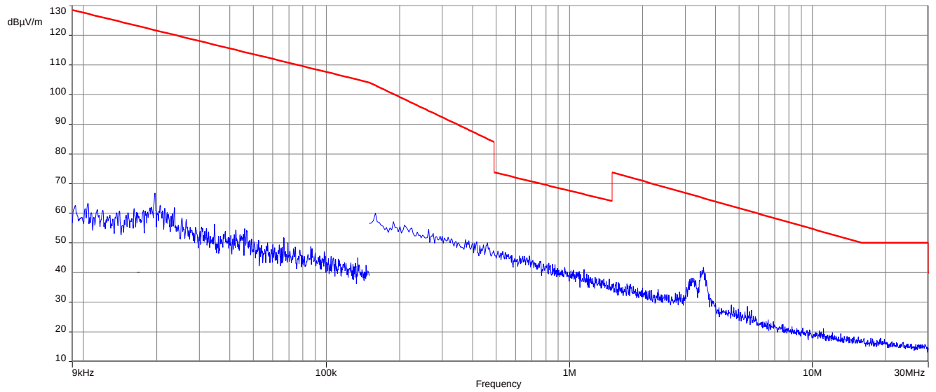
Plot 2: 9 kHz to 30 MHz, 2440 MHz, transmit mode, Antenna 1
