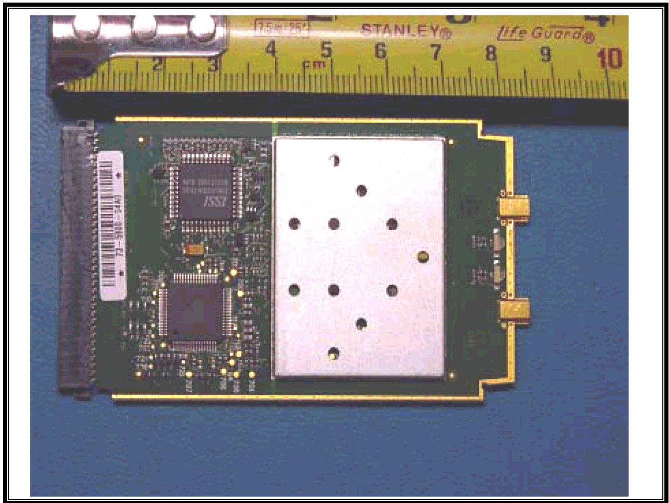
PHOTOGRAPH 29: FRONT VIEW OF PCB WITH SHIELD
