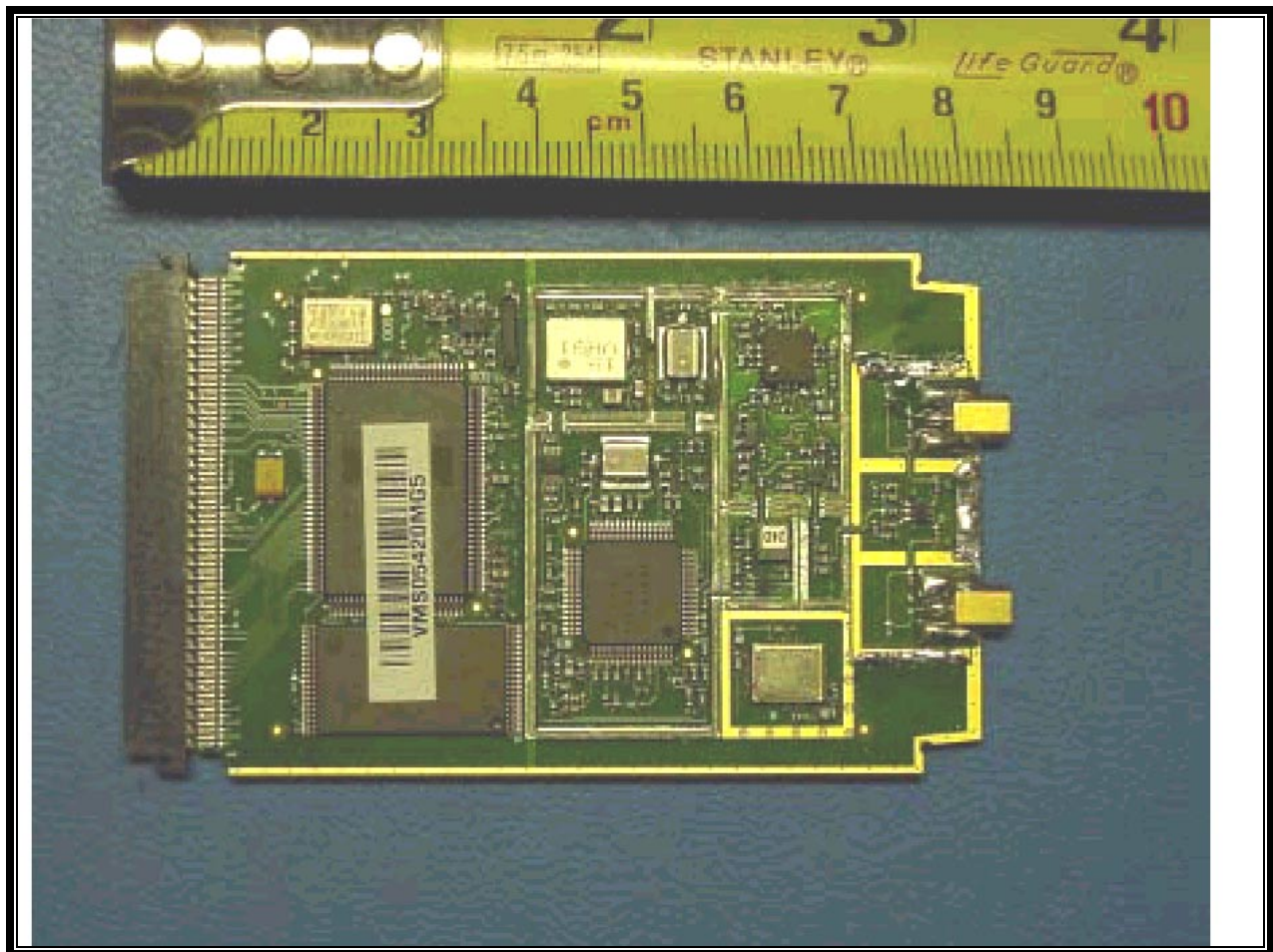
PHOTOGRAPH 32: BACK VIEW OF PCB WITHOUT SHIELD
