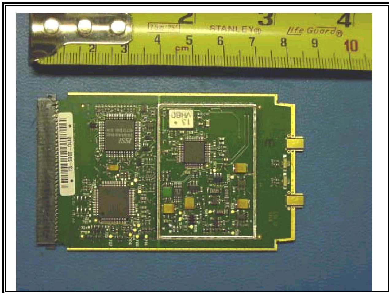
PHOTOGRAPH 30: FRONT VIEW OF PCB WITHOUT SHIELD
