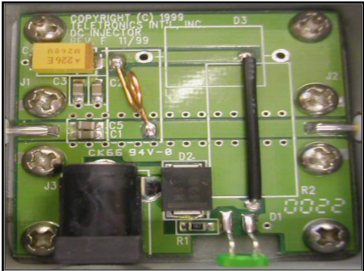
PHOTOGRAPH 33: FRONT VIEW PCB FROM DC INJECTOR
