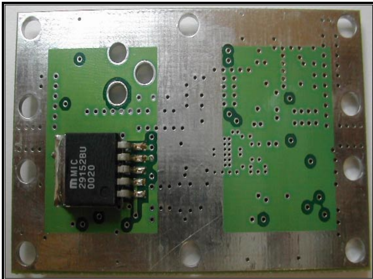
PHOTOGRAPH 36: REAR VIEW PCB FROM 500mW AMPLIFIER
