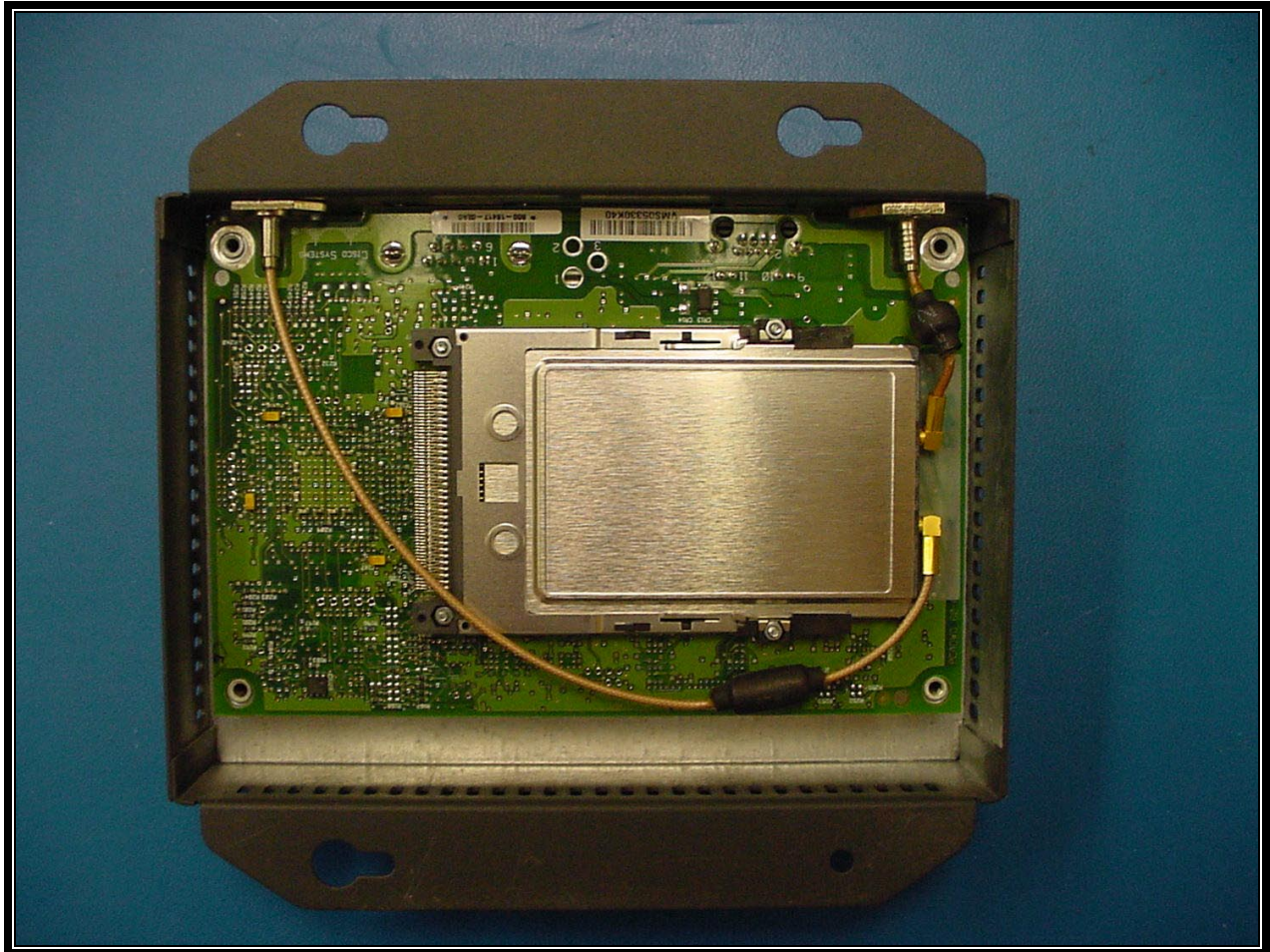
PHOTOGRAPH 26: INSIDE VIEW OF THE ACCESS POINT
