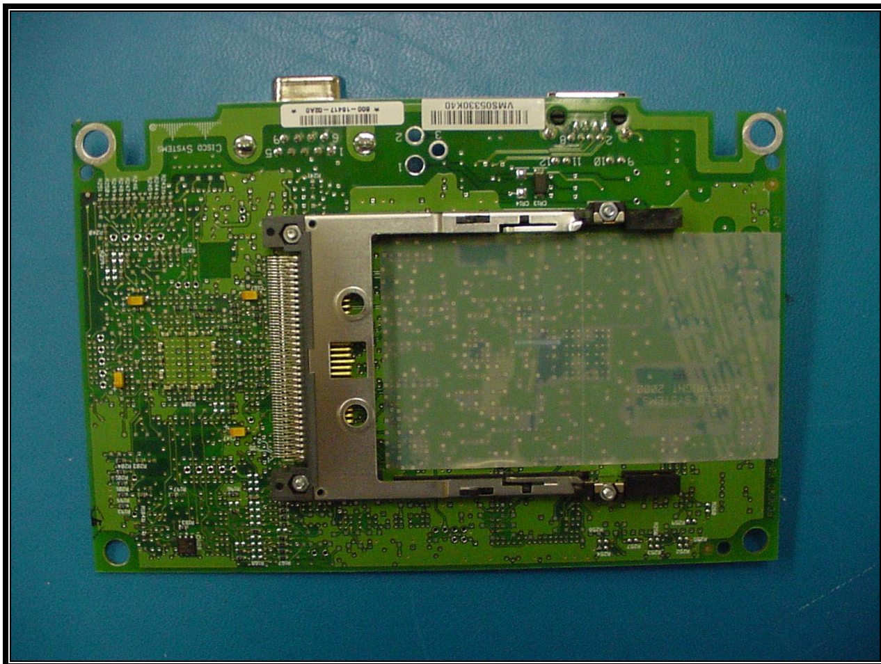
PHOTOGRAPH 28: REAR VIEW DIGITAL PART OF THE ACCESS POINT
