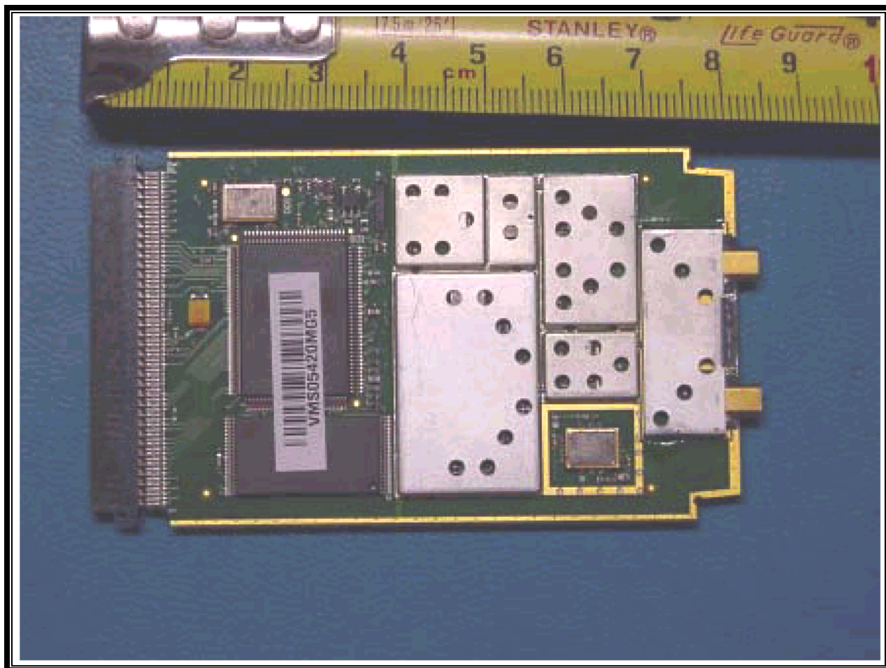
PHOTOGRAPH 31: BACK VIEW OF PCB WITH SHIELD
