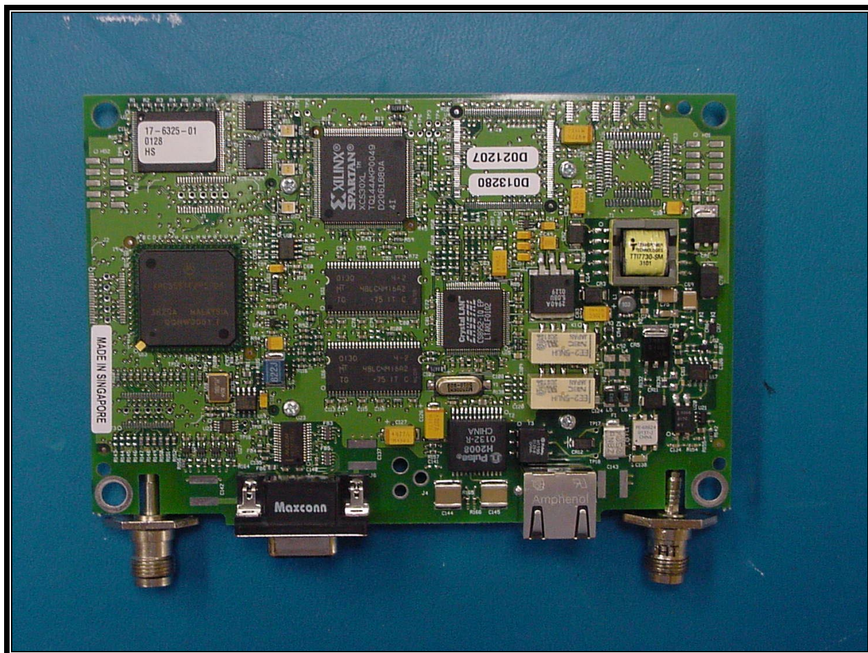
PHOTOGRAPH 27: FRONT VIEW DIGITAL PART OF THE ACCESS POINT
