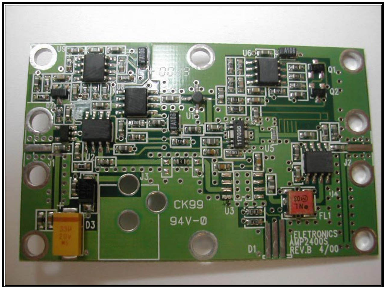
PHOTOGRAPH 35: FRONT VIEW PCB FROM 500mW AMPLIFIER
