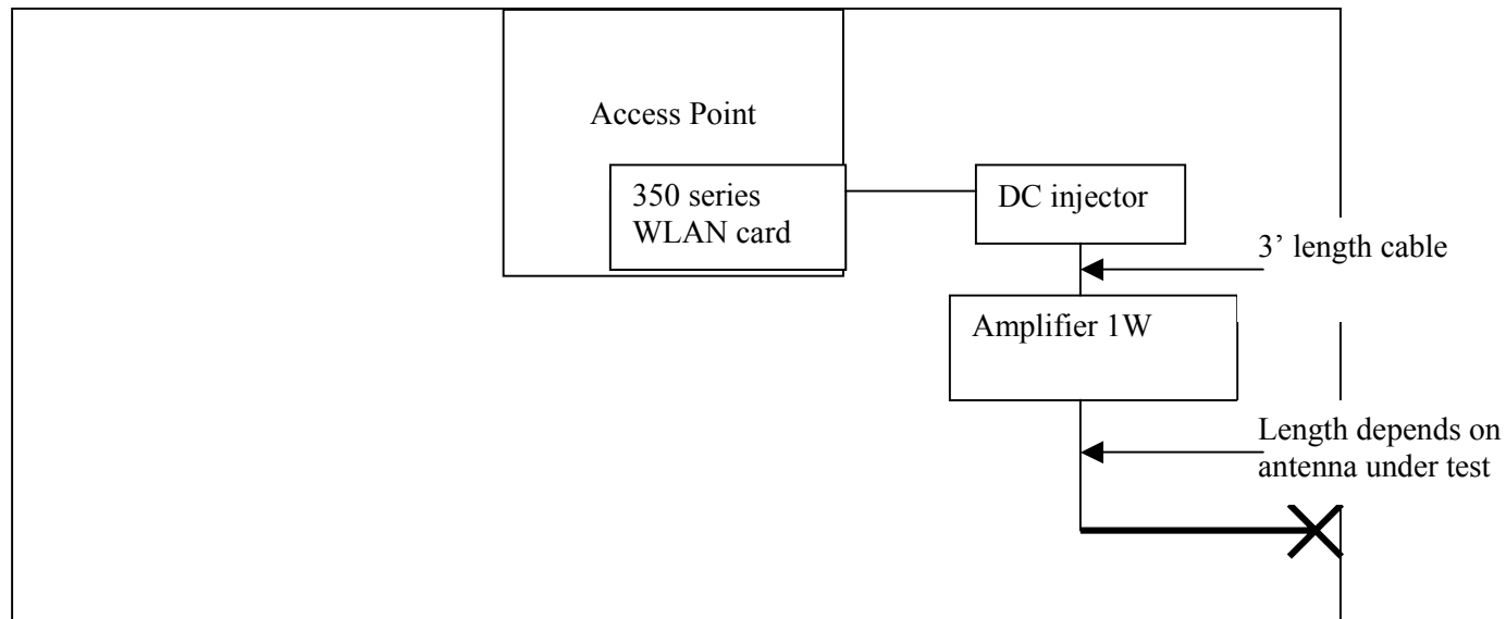
FIGURE 1: WORST CASE CONFIGURATION OF SYSTEM UNDER TEST
