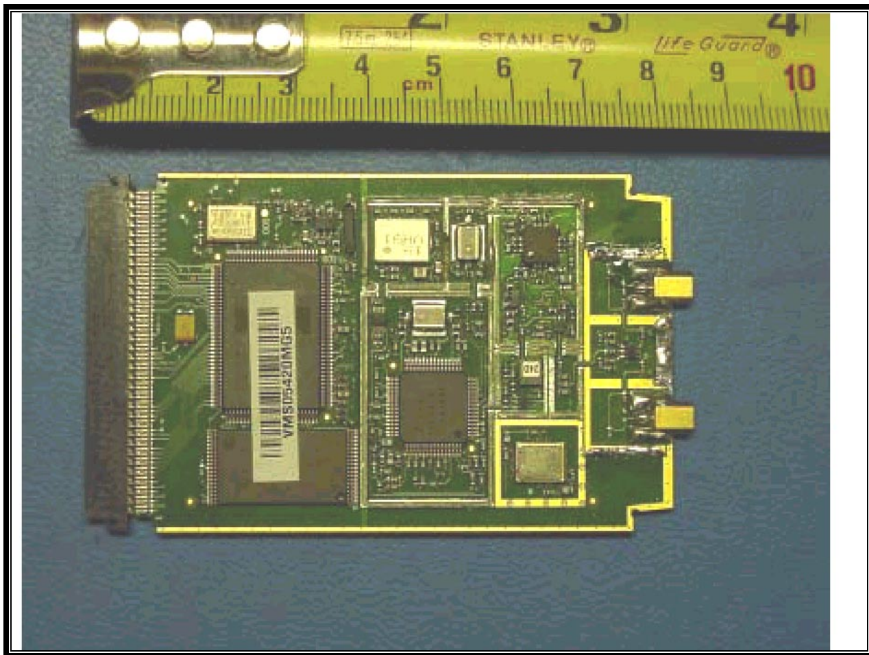
PHOTOGRAPH 29: BACK VIEW OF THE PCB WITHOUT SHIELD
