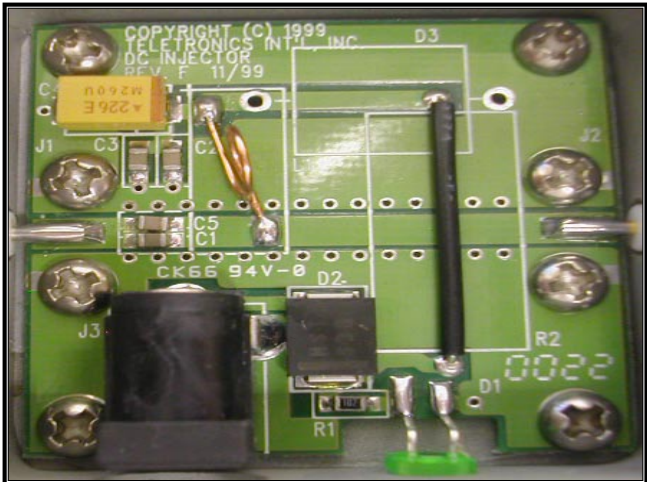
PHOTOGRAPH 30: FRONT VIEW PCB FROM DC INJECTOR
