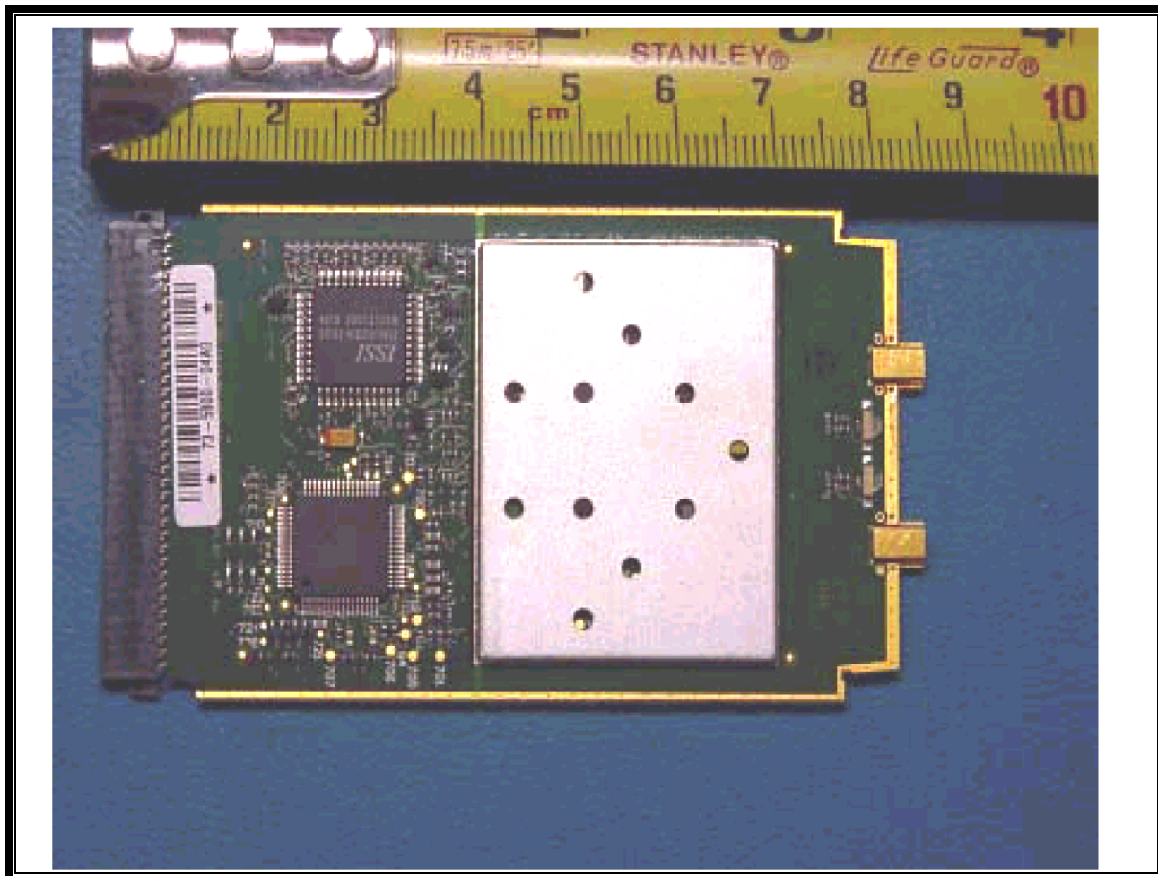
PHOTOGRAPH 26: FRONT VIEW OF THE PCB WITH SHIELD
