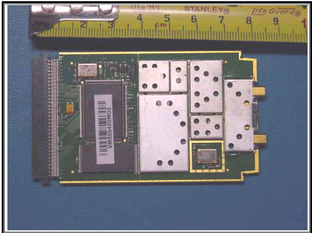
PHOTOGRAPH 28: BACK VIEW OF THE PCB WITH SHIELD
