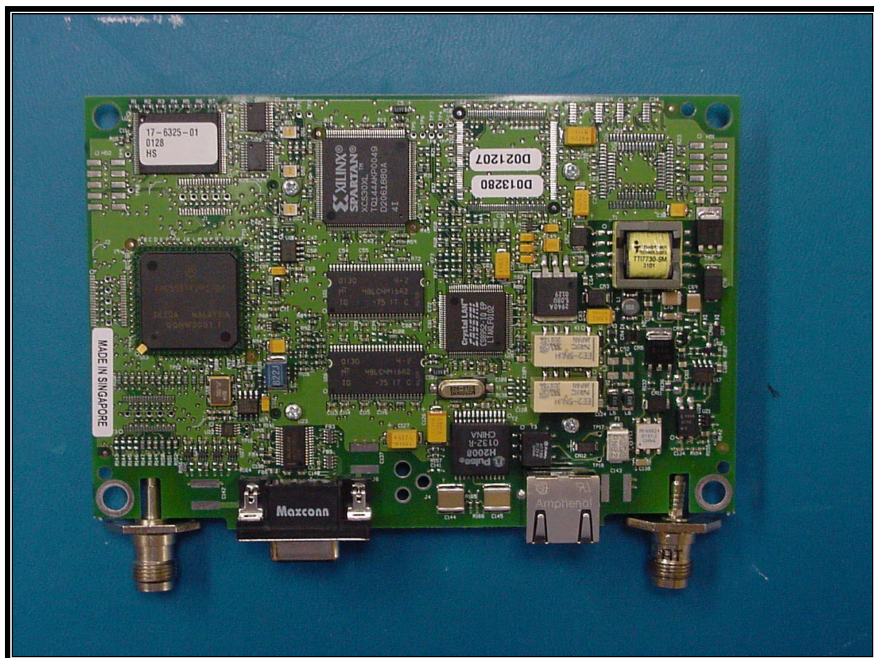
PHOTOGRAPH 24: FRONT VIEW DIGITAL PART OF THE ACCESS POINT
