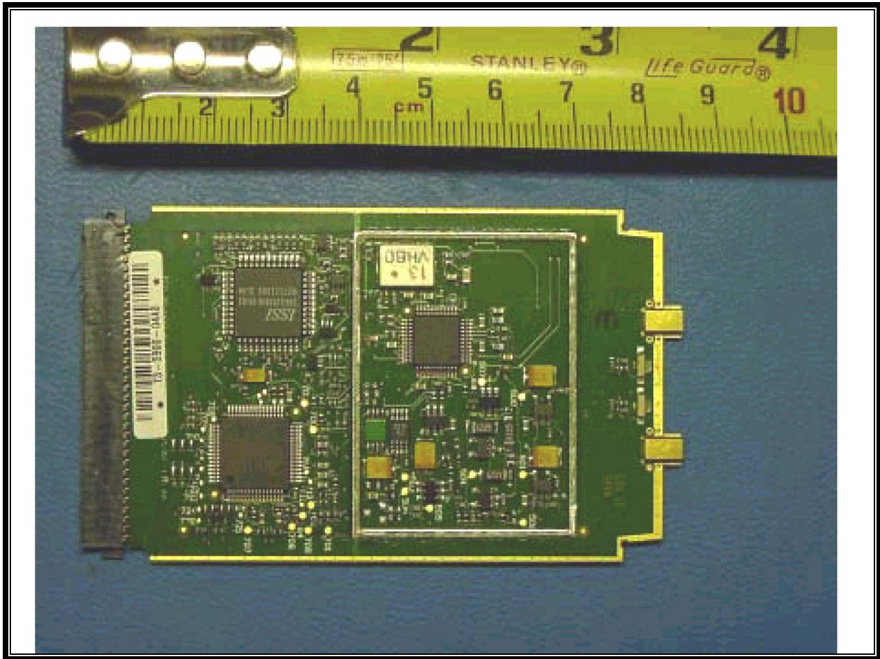
PHOTOGRAPH 27: FRONT VIEW OF THE PCB WITHOUT SHIELD
