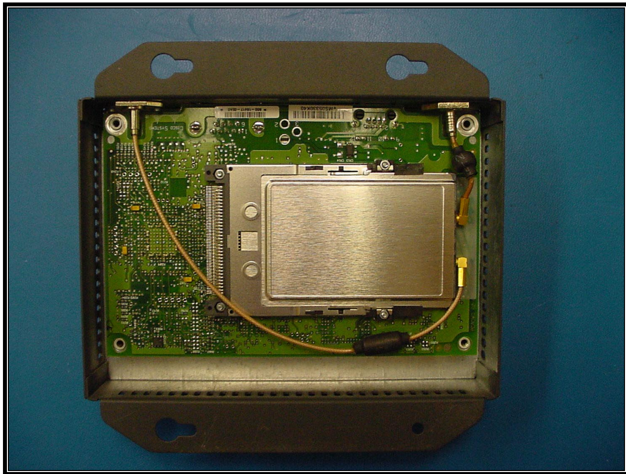
PHOTOGRAPH 23: INSIDE VIEW OF THE ACCESS POINT
