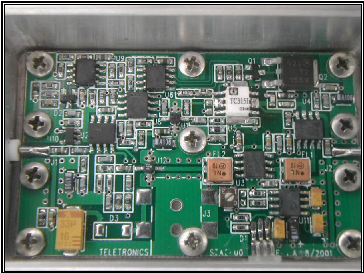
PHOTOGRAPH 31: FRONT VIEW PCB FROM 1W AMPLIFIER
