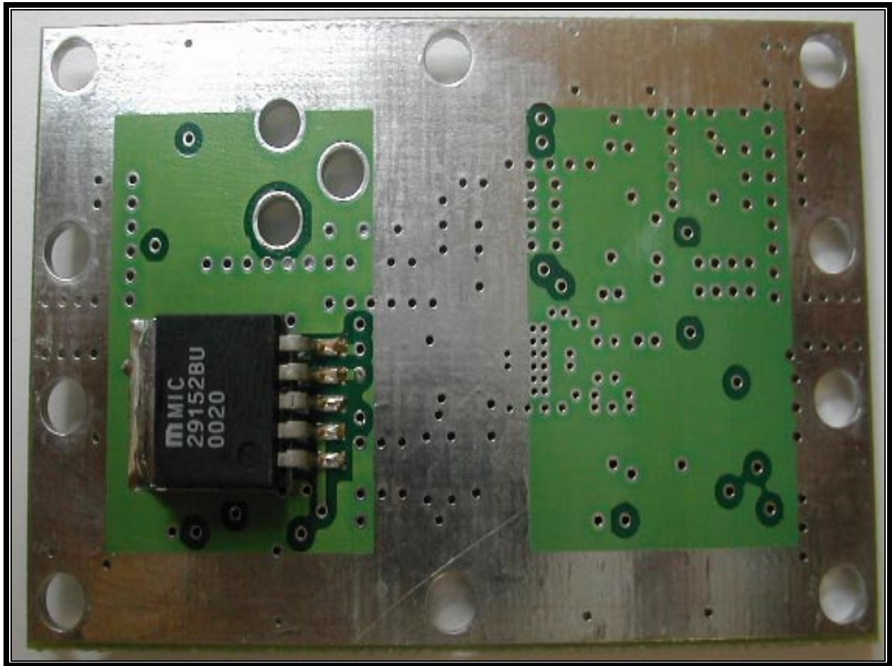
PHOTOGRAPH 32: REAR VIEW PCB FROM 1W AMPLIFIER
