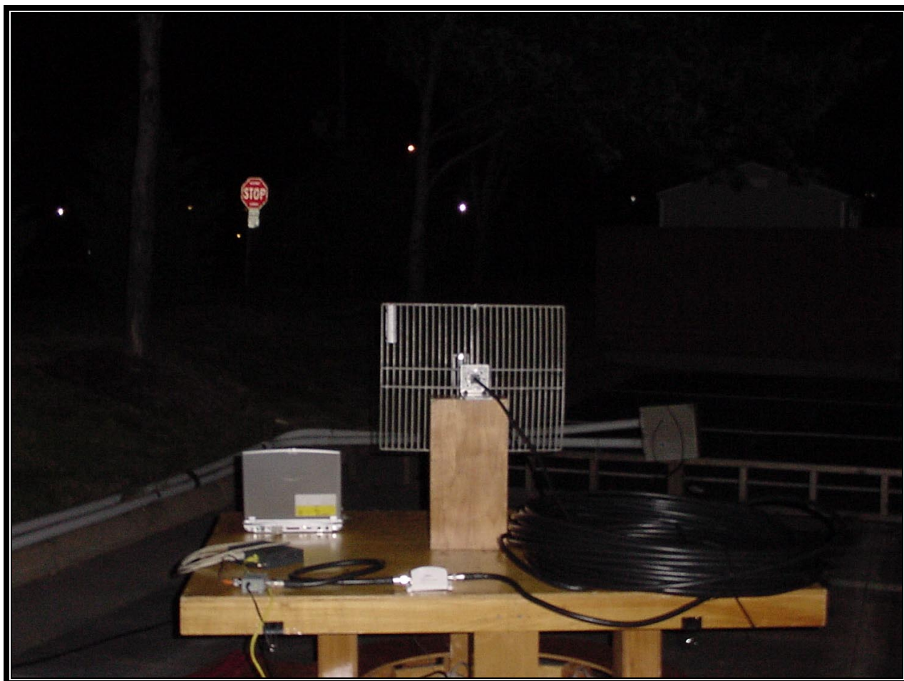
PHOTOGRAPH 15: RADIATED EMISSIONS REAR VIEW WORST CASE CONFIGURATION 18 dBi Grid
