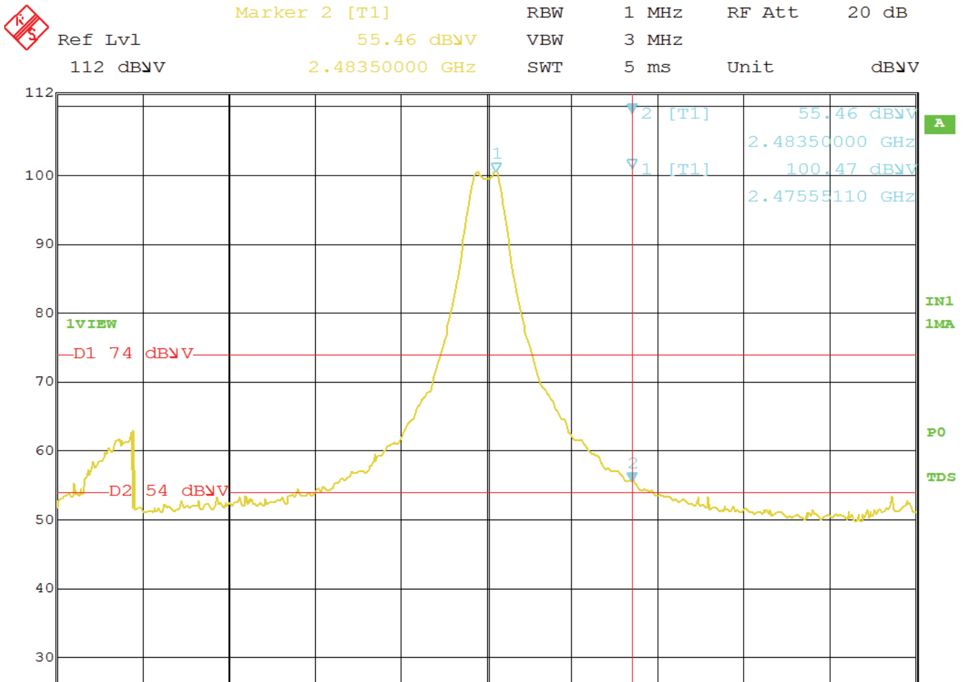
Band Edge – Vertical Polarization – High Ch – Y-Axis – Worst Case
