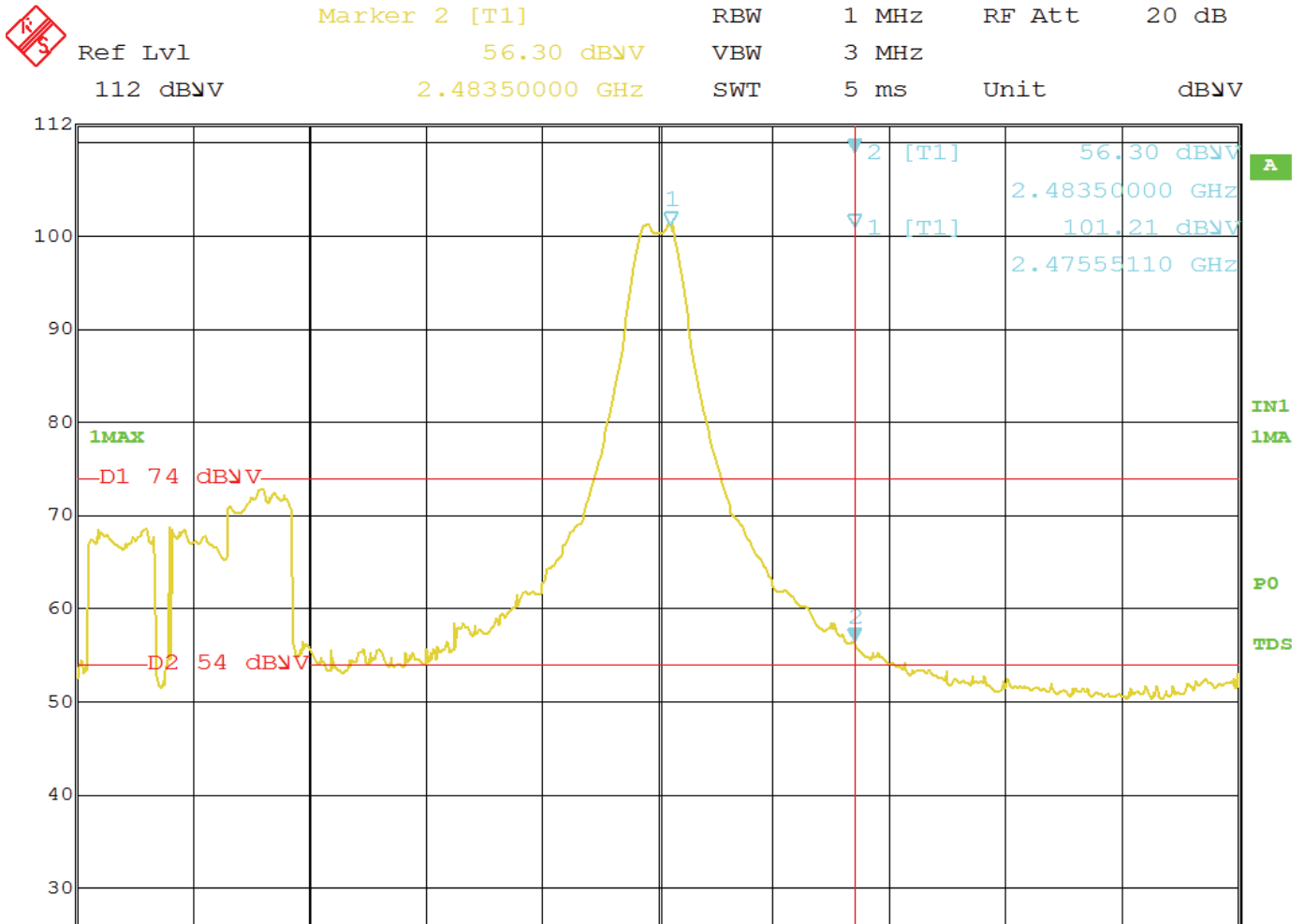
Band Edge – Horizontal Polarization – High Ch – X-Axis – Worst Case
