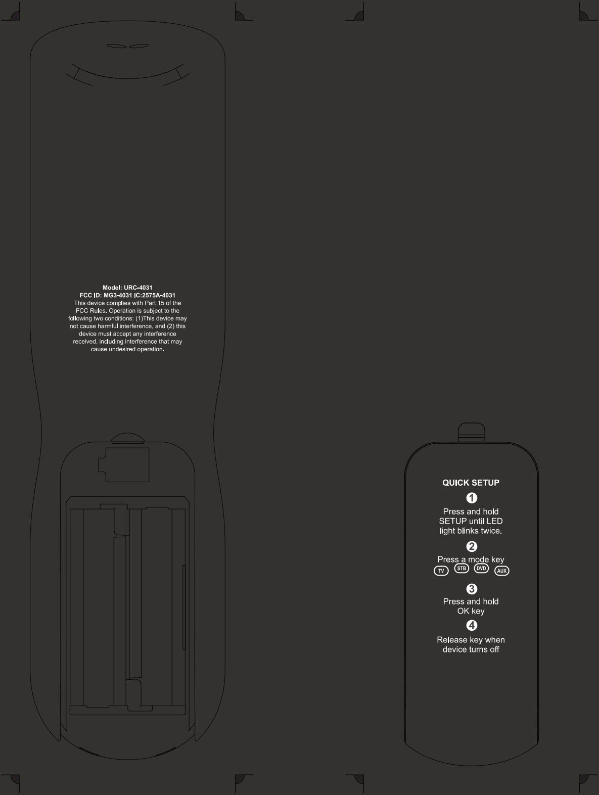
Backcase Artwork
