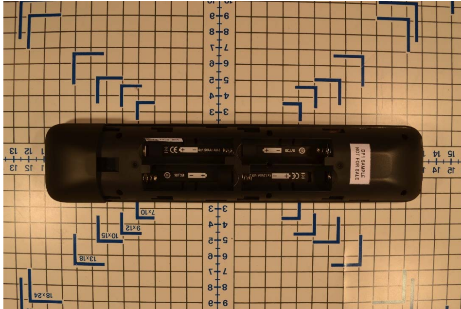
Battery Cover Removed
