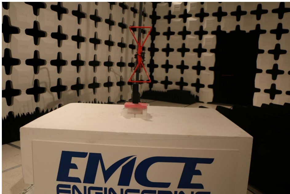
Radiated Emissions 30MHz – 1 GHz
