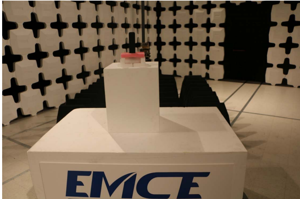
Radiated Emissions > 1 GHz
