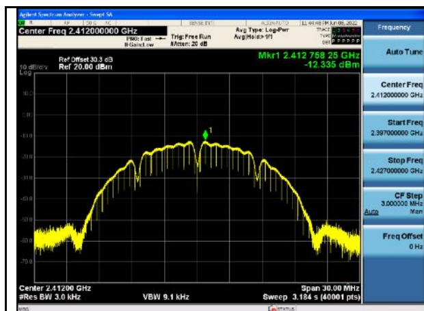
PSD-802.11b-Low CH
