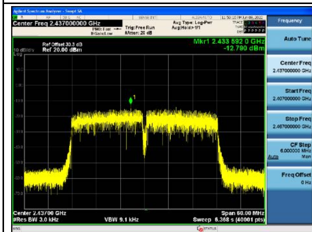
PSD-802.11n40-Mid CH
