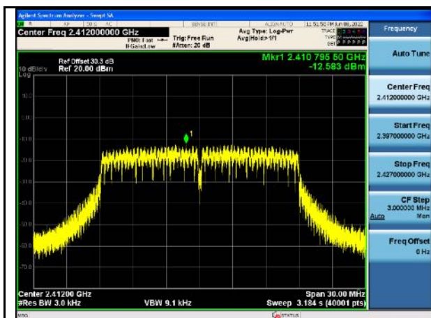
PSD-802.11n20-Low CH
