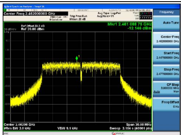
PSD-802.11g-High CH
