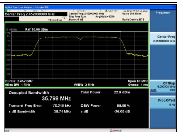
99%_802.11n40_High CH
