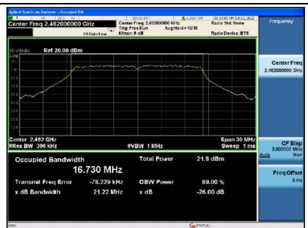
99%_802.11g_High CH
