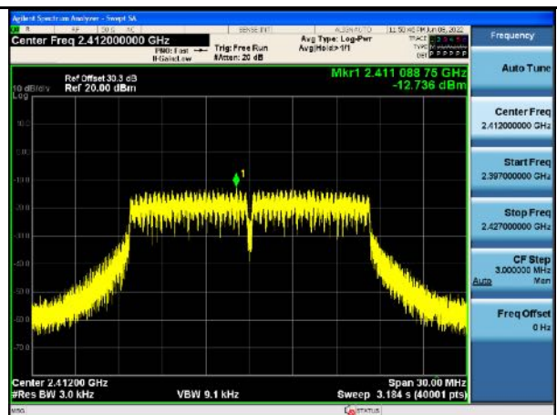
PSD-802.11g-Low CH
