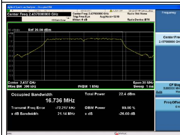
99%_802.11g_Mid CH
