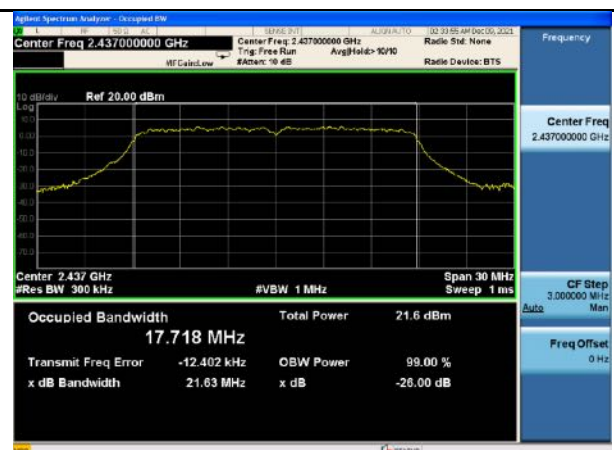
99%_802.11n20_Mid CH
