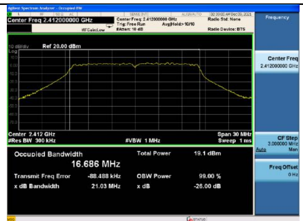
99%_802.11g_Low CH
