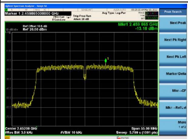
PSD-802.11n40-High CH
