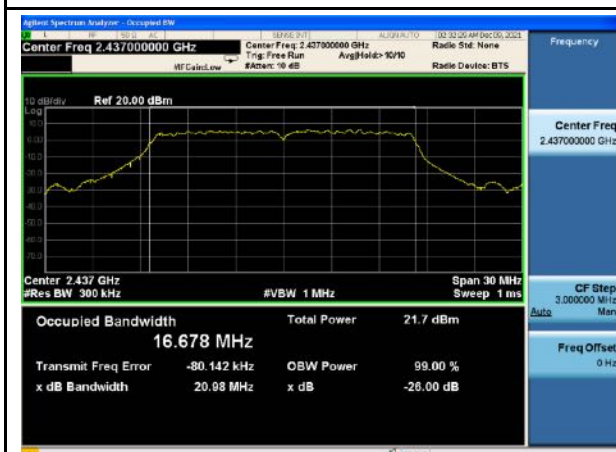
99%_802.11g_Mid CH
