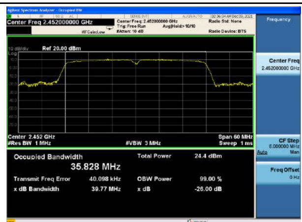
99%_802.11n40_High CH
