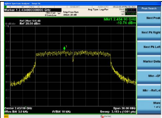
PSD-802.11n20-Mid CH
