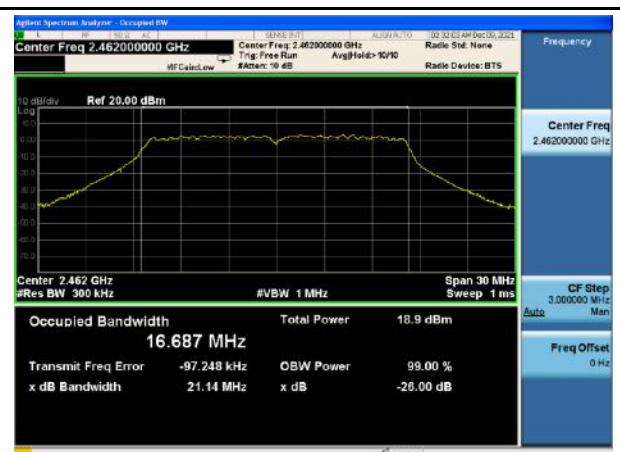
99%_802.11g_High CH
