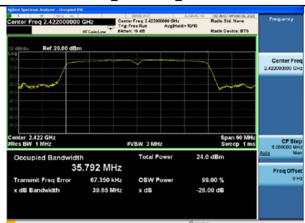
99%_802.11n40_Low CH
