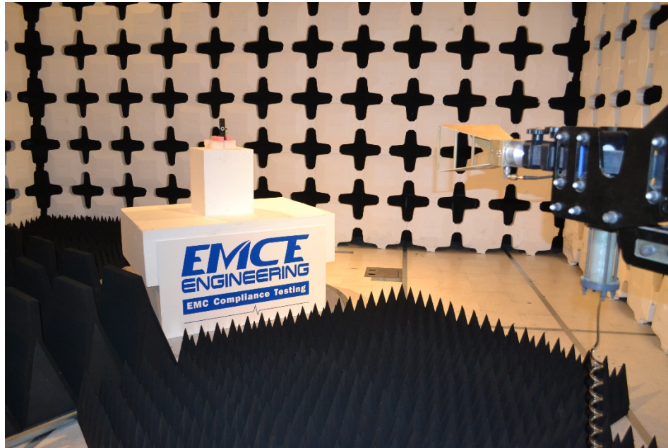
Radiated Emissions – Above 1 GHz
