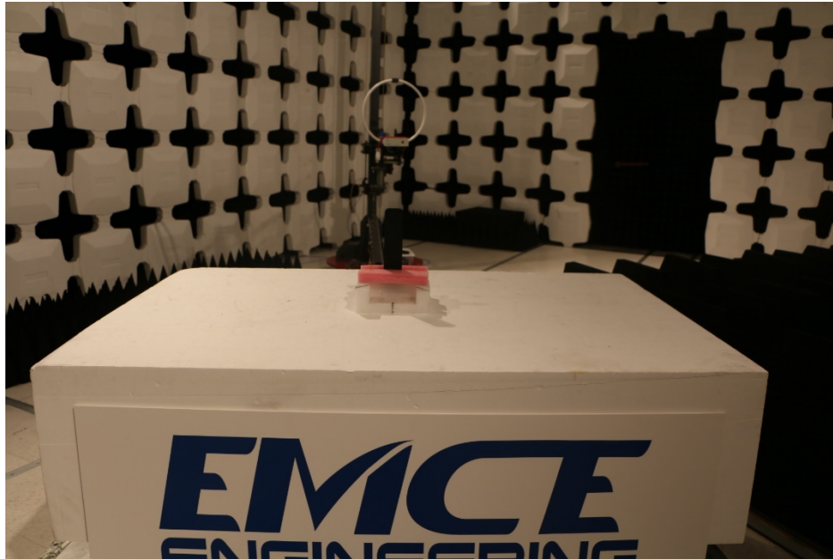
Radiated Emissions <30 MHz
