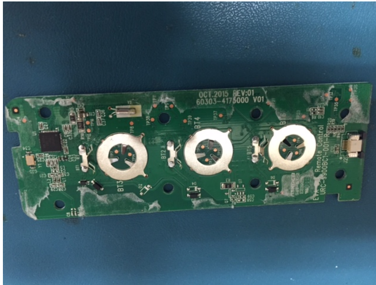
EUT Internal - PCB Top
