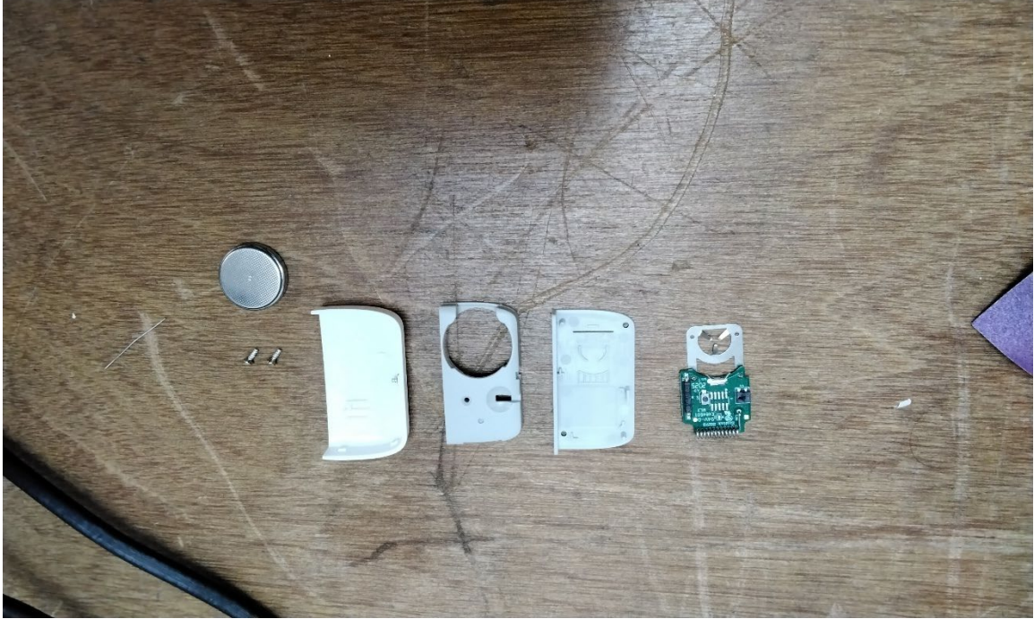
Internal Circuit Board - Top
