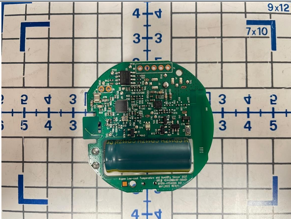
Mainboard View 2
