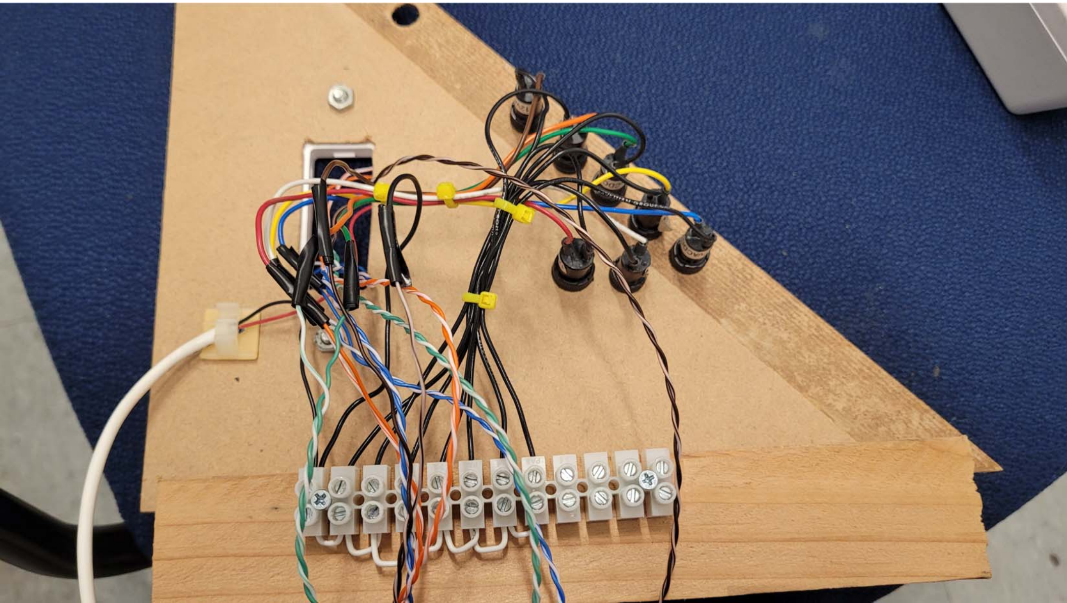
Mounting Device - Rear View
