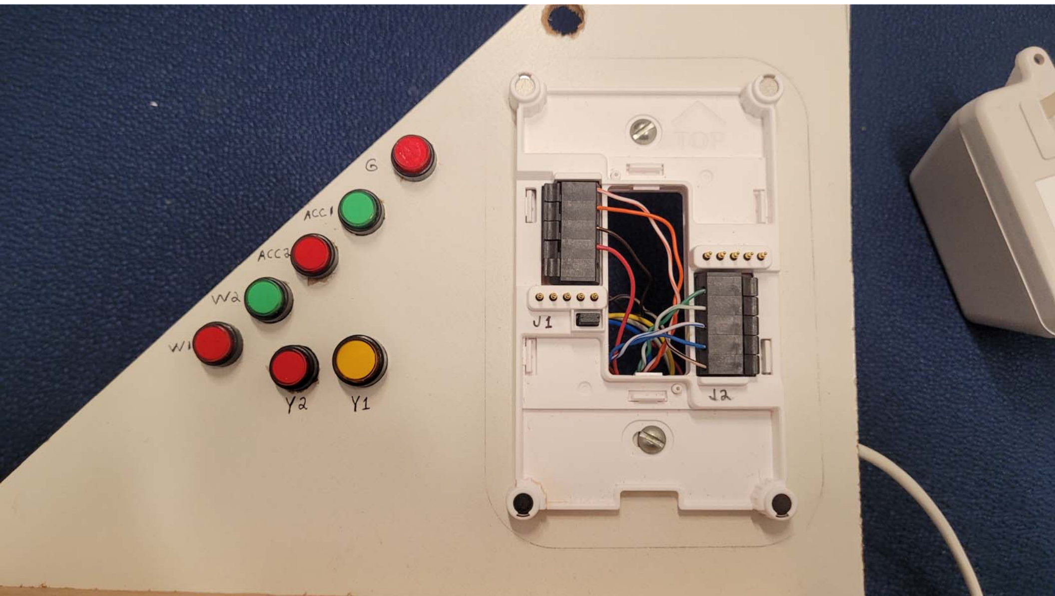
Mounting Device - Front View Note: Only used for testing and is not part of the EUT
