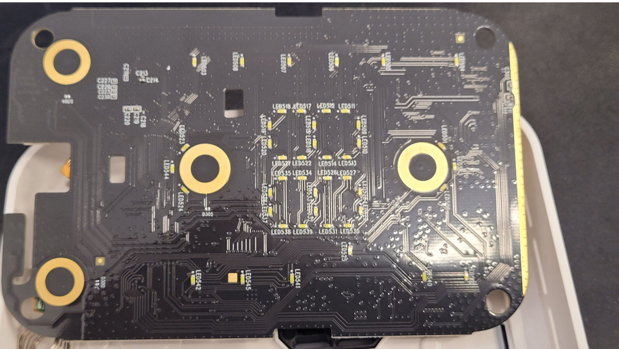
Bottom View of the PCB for the EUT - View #2
