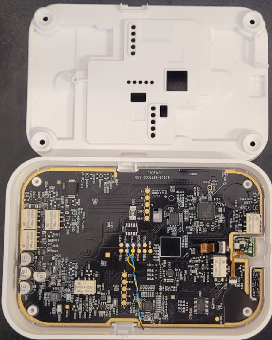
Inside View of the EUT
