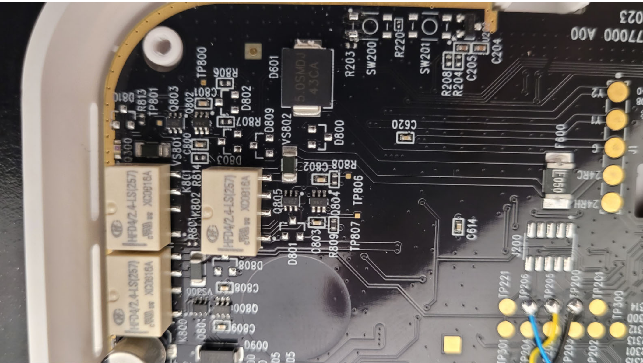
Top View of the PCB - Closeup #1
