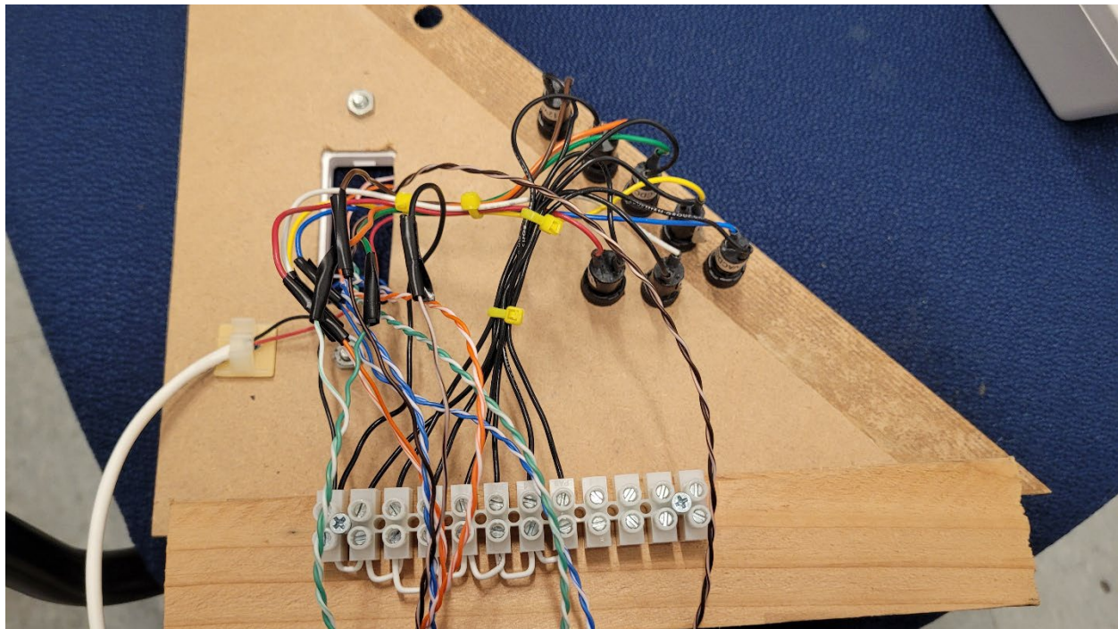
Back View of the Mounting Device (Note Only used for testing and not part of the EUT)
