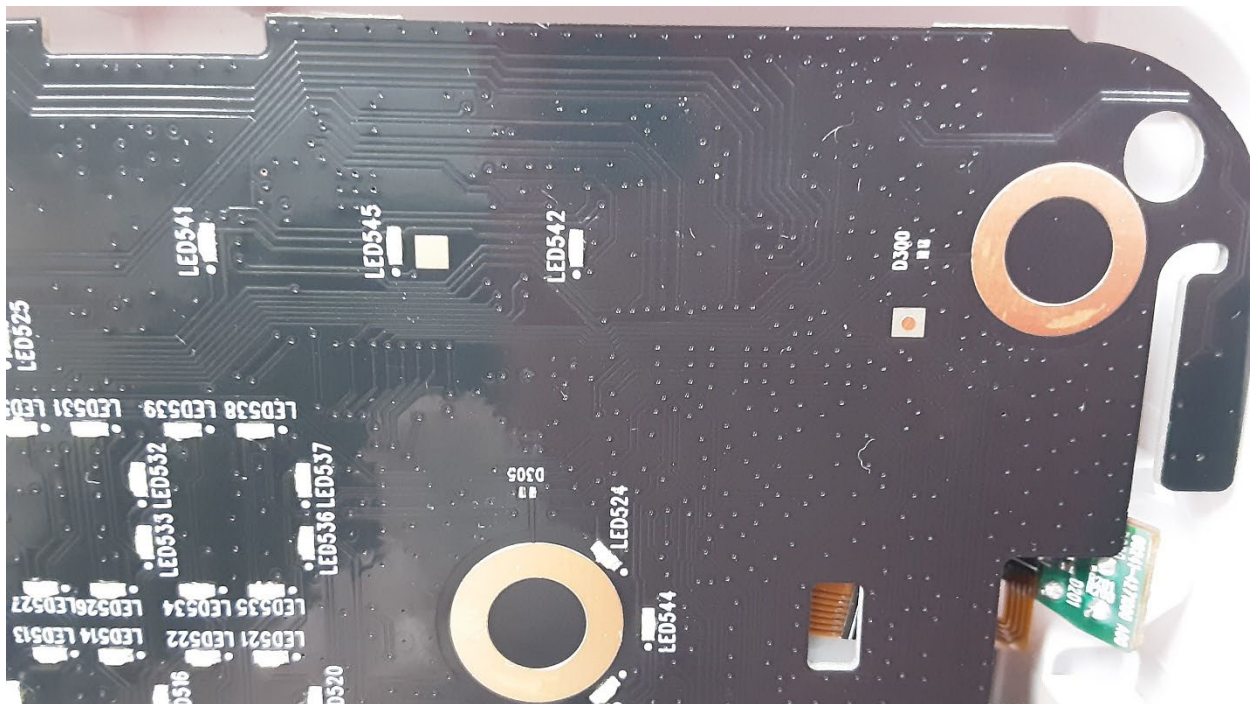
Bottom View of the PCB – Close up #2
