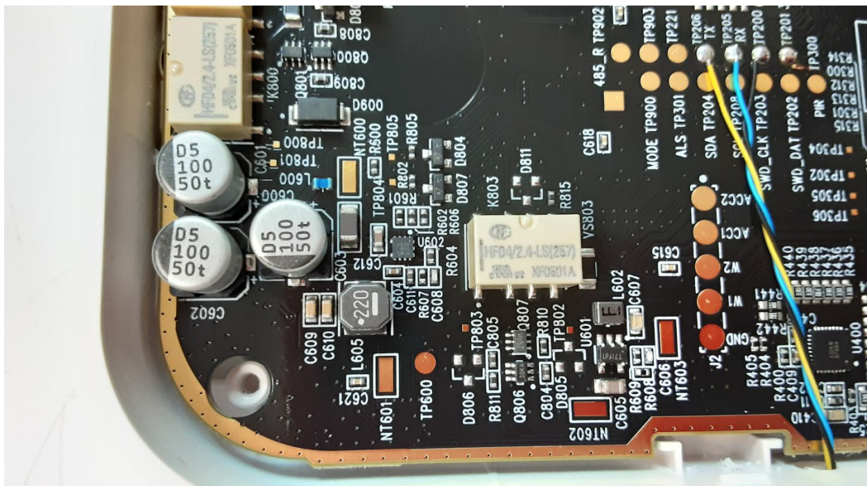
Top View of the PCB – Close up #4
