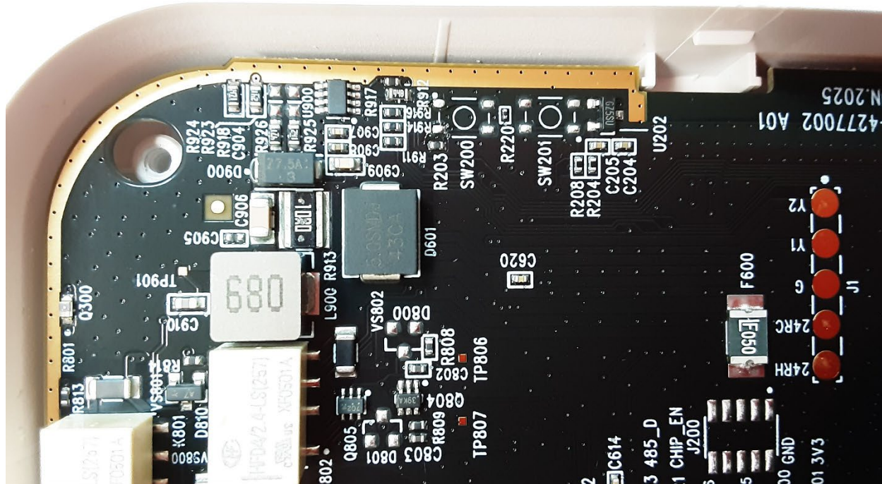
Top View of the PCB – Close up #1
