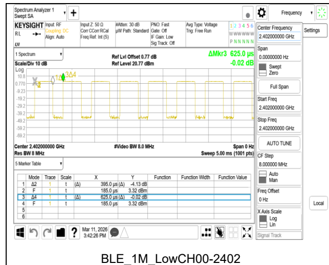
BLE_1M_LowCH00-2402
