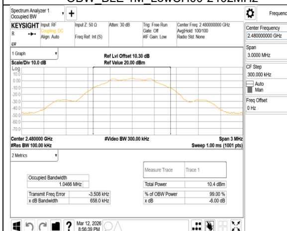
OBW_BLE 1M_HighCH39-2480MHz
