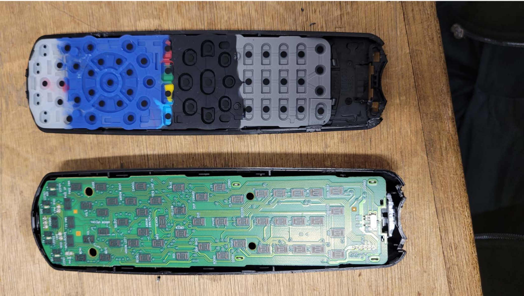
Inside View of the EUT
