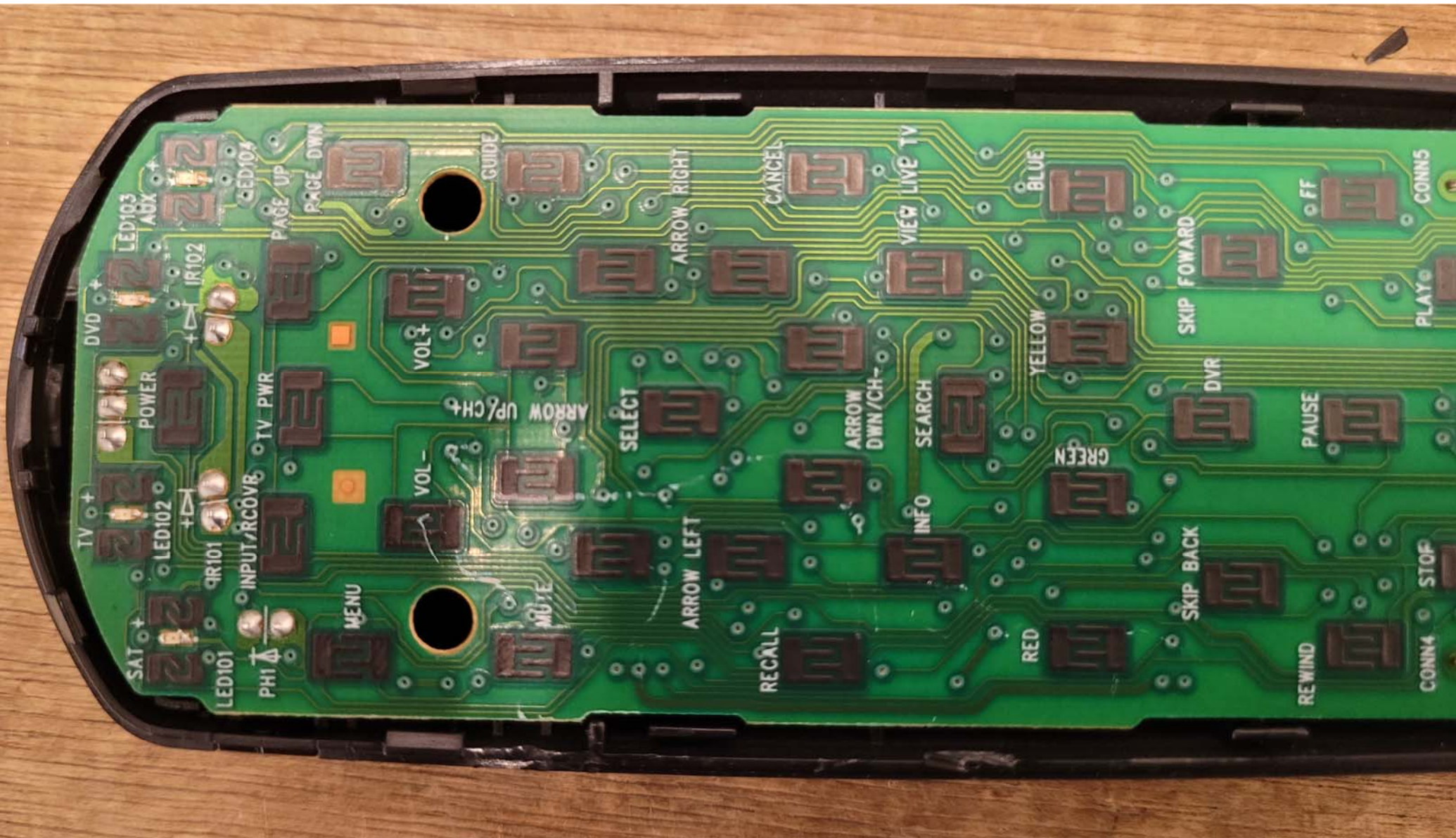
Top View of the PCB - Closeup #1
