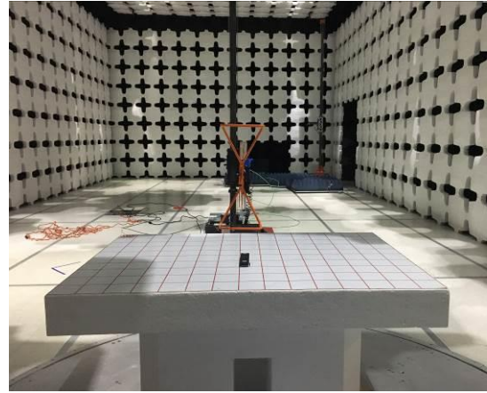
Radiated Emissions (<1GHz) – Rear View
