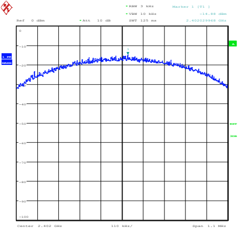
2402 MHz
