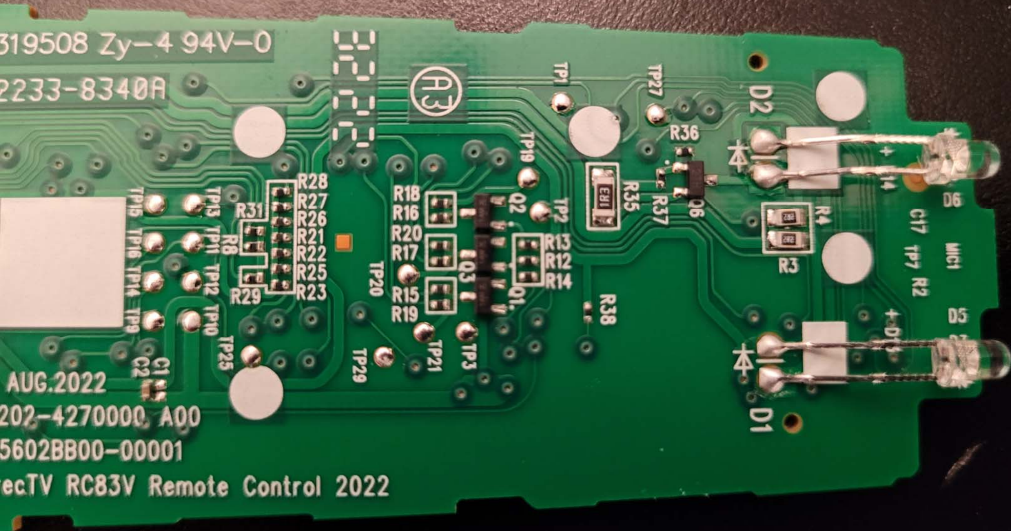
Top View of the PCB - Closeup #3
