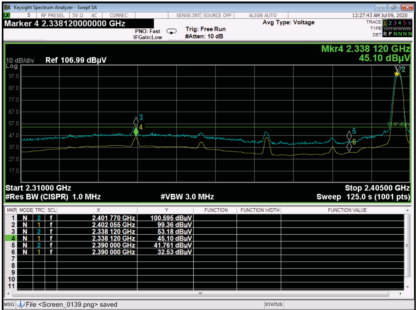
Band Edge – Low Channel – Vertical Polarization – Y-Axis
