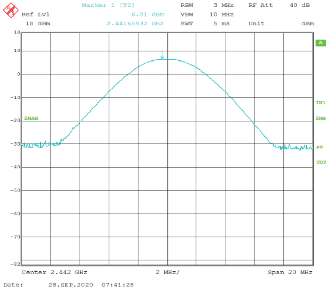
Peak Output Power – Middle Channel
