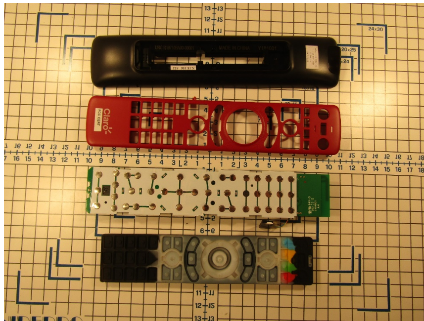
EUT – Internal
