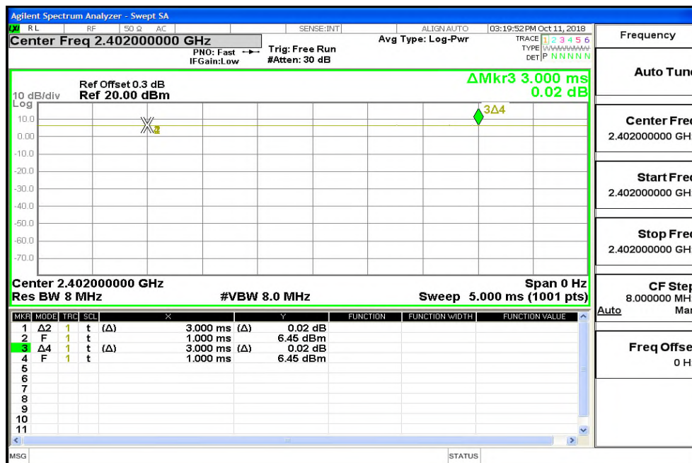
Duty Cycle_BLE_1M_LowCH00-2402
