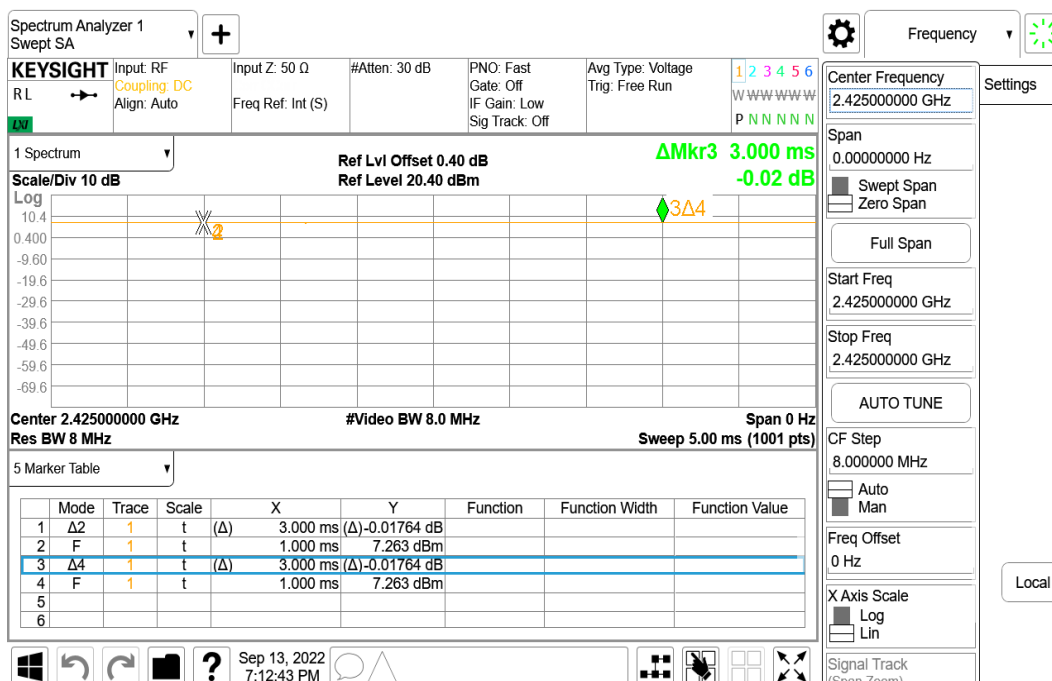
Zigbee_LowCH15-2425
