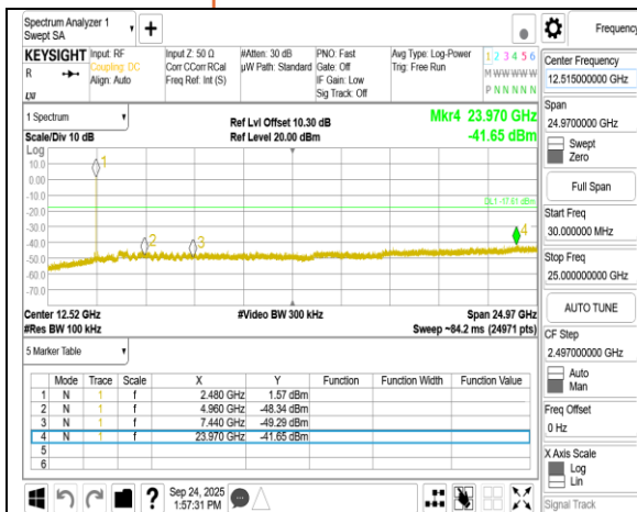
Spurious Emission_BLE 1M_HighCH39-2480MHz
