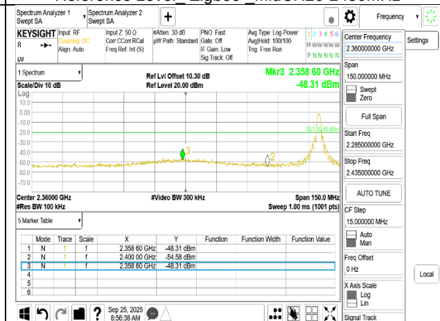
Band Edge Zigbee LowCH15-2425MHz
