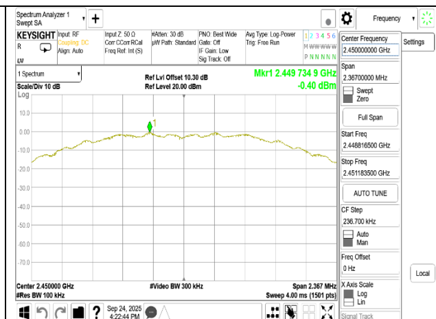
Reference Level Zigbee MidCH20-2450MHz
