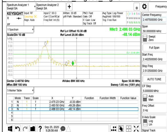
Band Edge Zigbee HighCH25-2475MHz
