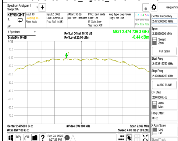
Reference Level Zigbee HighCH25-2475MHz
