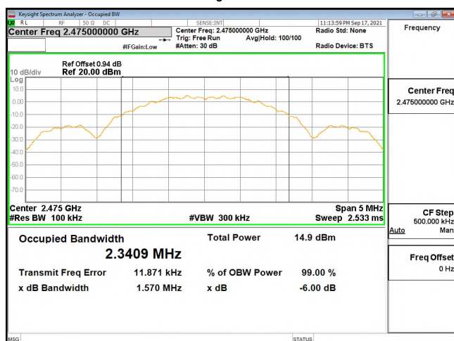
OBW_HighCH25-2475
