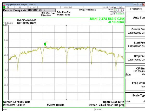
PSD_HighCH25-2475
