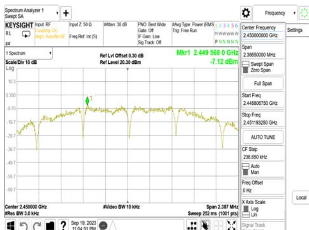
PSD_Zigbee_MidCH20-2450MHz
