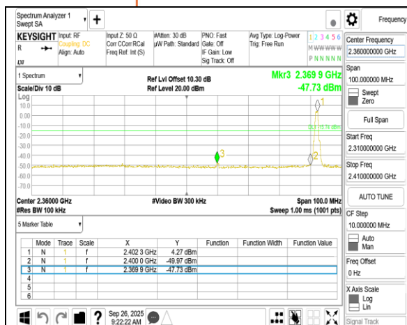
Band Edge_BLE 1M_LowCH00-2402MHz
