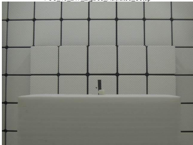
FCC_15_247_ZigBee_Radiated_Setup
