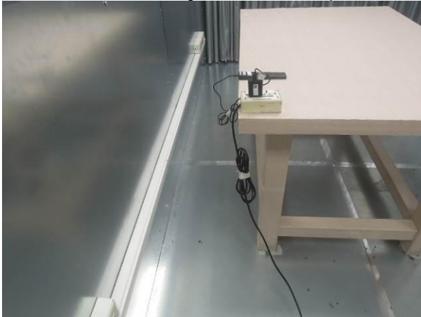
FCC_15_247_ZigBee_Conduction_Setup
