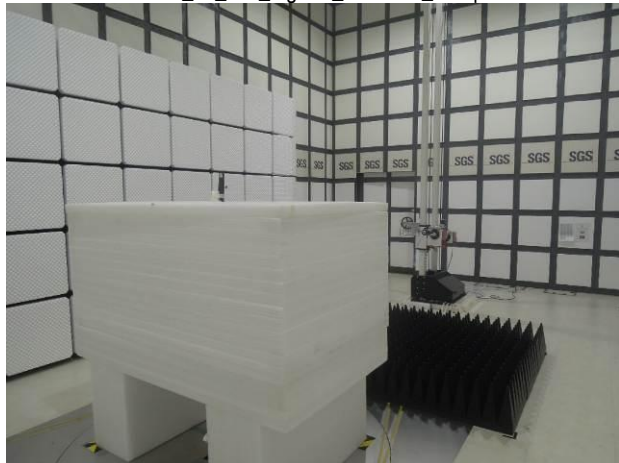
FCC_15_247_ZigBee_Radiated_Setup
