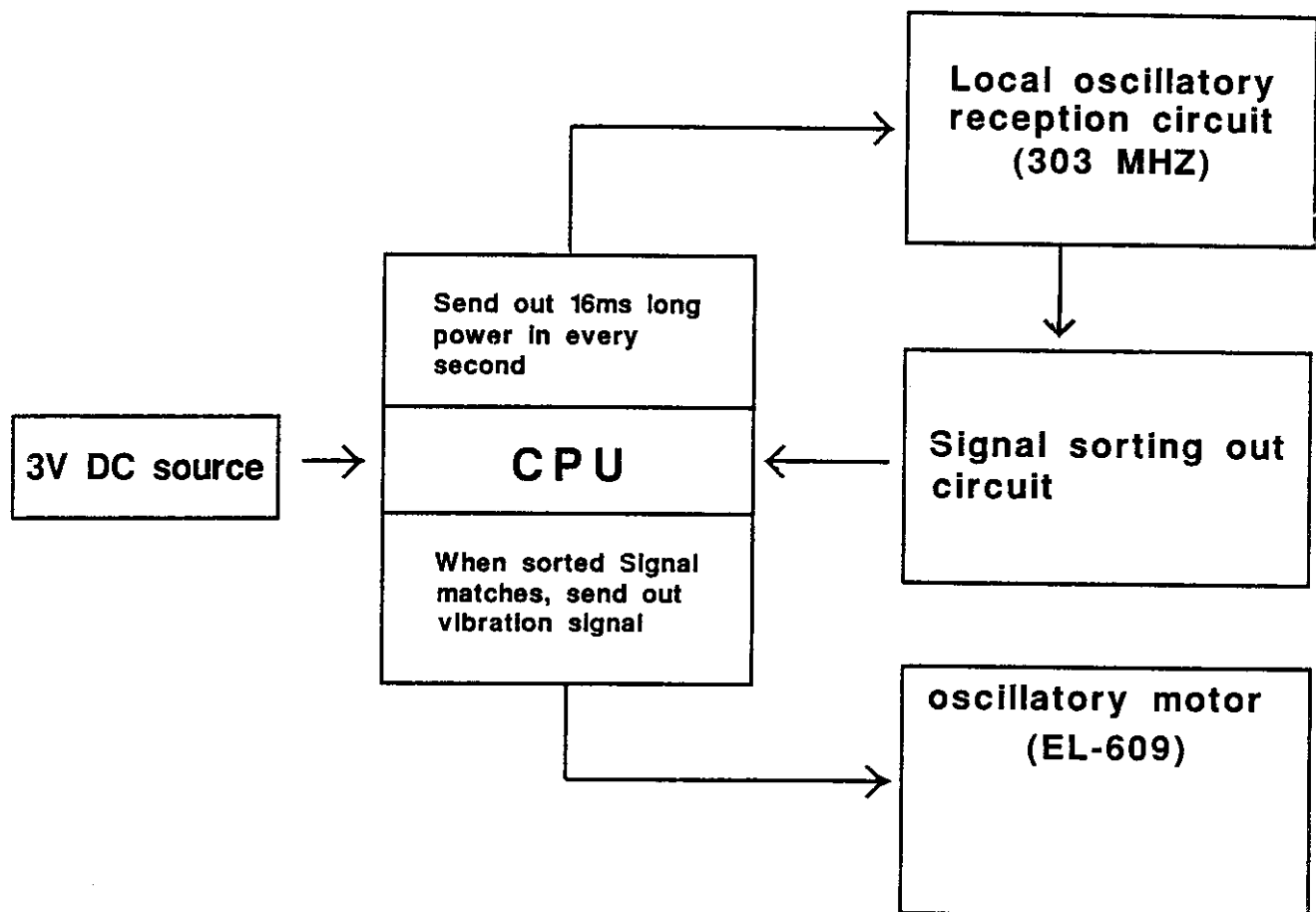
Schematic Diagram of Receiver
