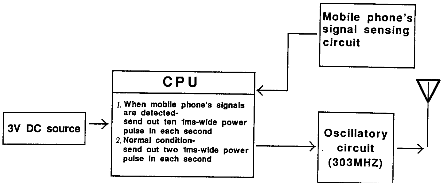
Schematic Diagram of Transmitter
