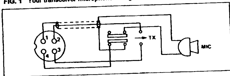
4 Wire Mic. Cable
