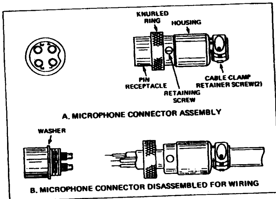
FIG. 3 Microphone plug wiring.
