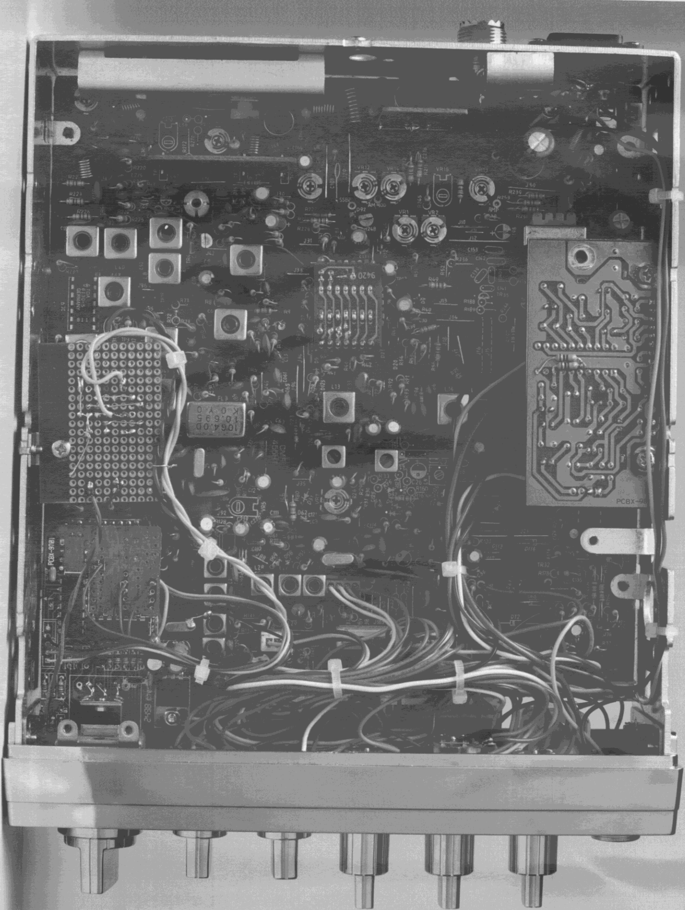
NR-150 CB Mobile Radio - Main Board Side 1
